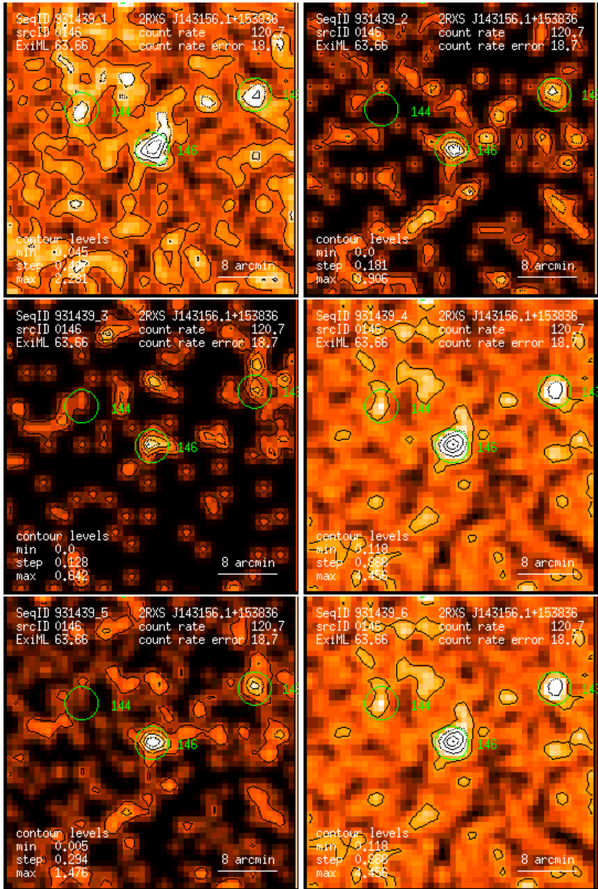
Figure 146: RASS 931439: detection 0146: band rate images, Gaussian filter: (1) PSPC channels 11 – 41, (2) 52 – 90, (3) 91 – 201, (4) 11 – 235, (5) 52 – 201, (6) 11 – 201. Broad band rates in counts/ks. Band rate contour levels in counts/ks/arcmin 2 .
