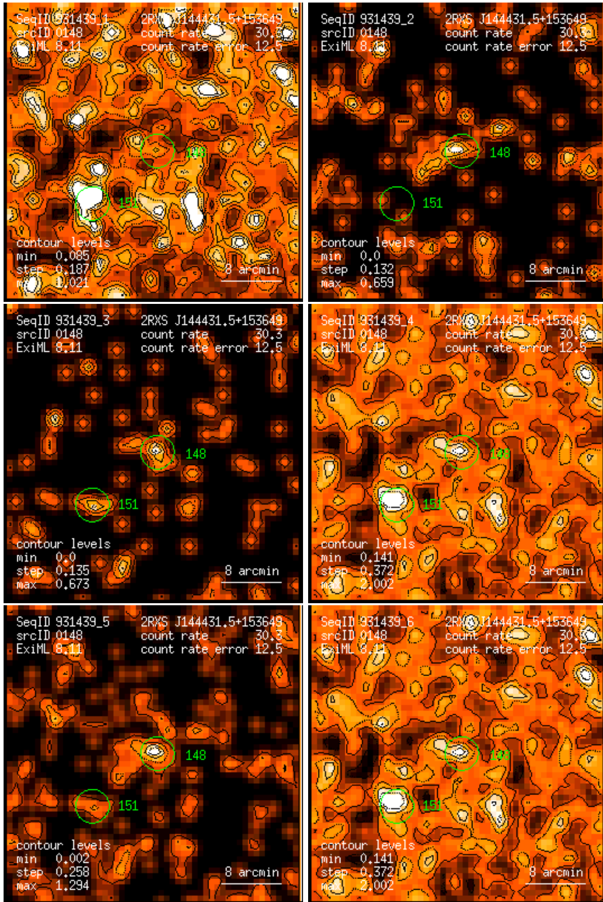
Figure 148: RASS 931439: detection 0148: band rate images, Gaussian filter: (1) PSPC channels 11 – 41, (2) 52 – 90, (3) 91 – 201, (4) 11 – 235, (5) 52 – 201, (6) 11 – 201. Broad band rates in counts/ks. Band rate contour levels in counts/ks/arcmin 2 .
