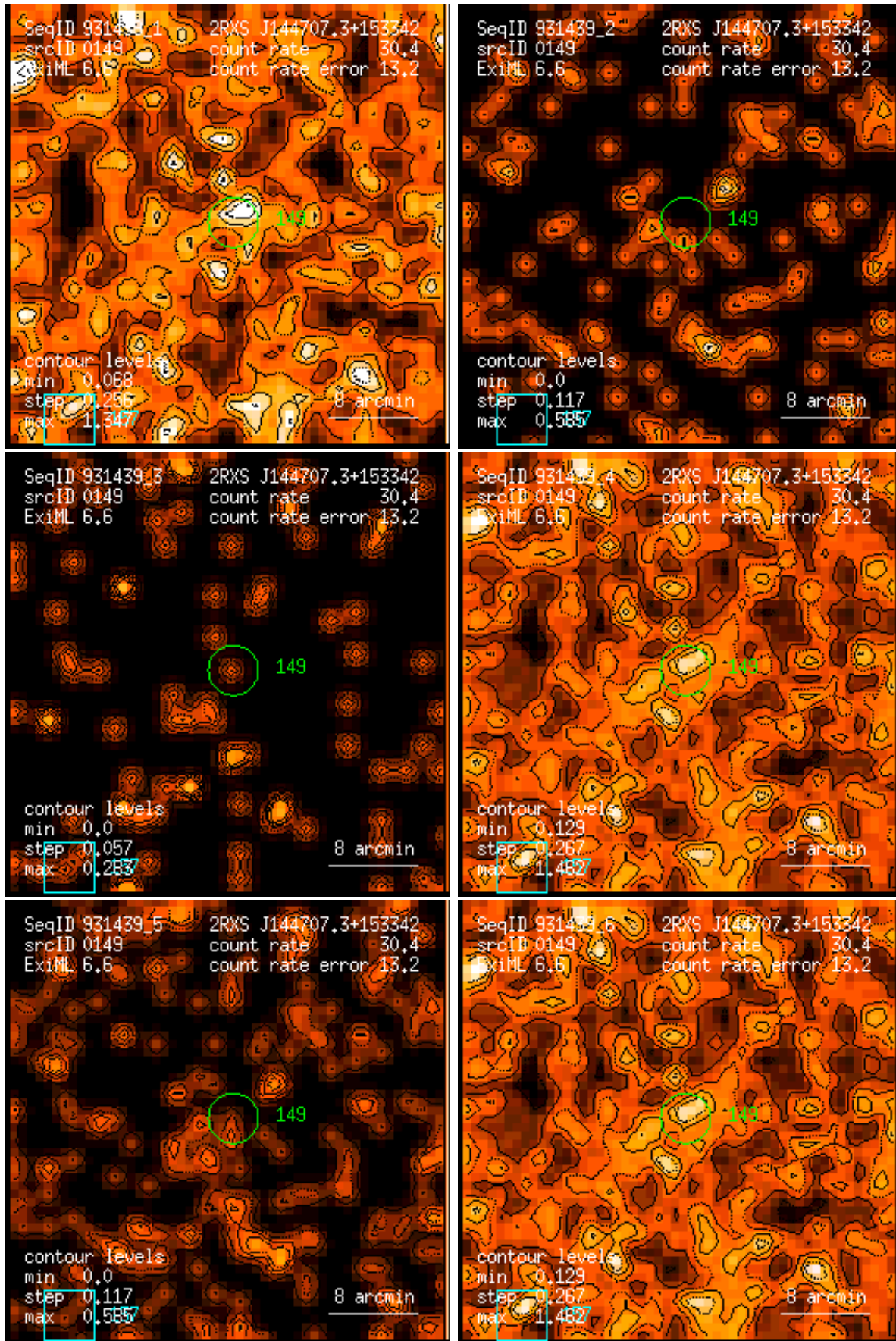
Figure 149: RASS 931439: detection 0149: band rate images, Gaussian filter: (1) PSPC channels 11 – 41, (2) 52 – 90, (3) 91 – 201, (4) 11 – 235, (5) 52 – 201, (6) 11 – 201. Broad band rates in counts/ks. Band rate contour levels in counts/ks/arcmin 2 .
