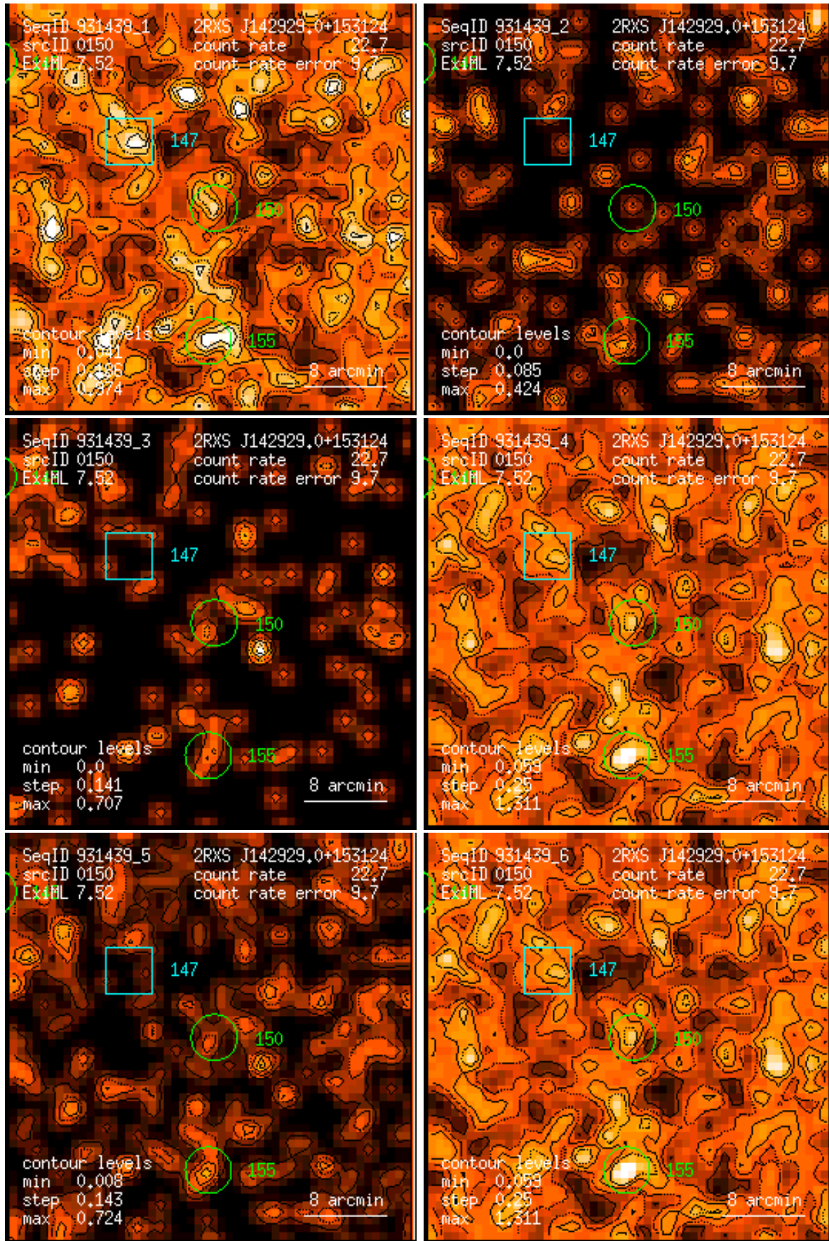
Figure 150: RASS 931439: detection 0150: band rate images, Gaussian filter: (1) PSPC channels 11 – 41, (2) 52 – 90, (3) 91 – 201, (4) 11 – 235, (5) 52 – 201, (6) 11 – 201. Broad band rates in counts/ks. Band rate contour levels in counts/ks/arcmin 2 .
