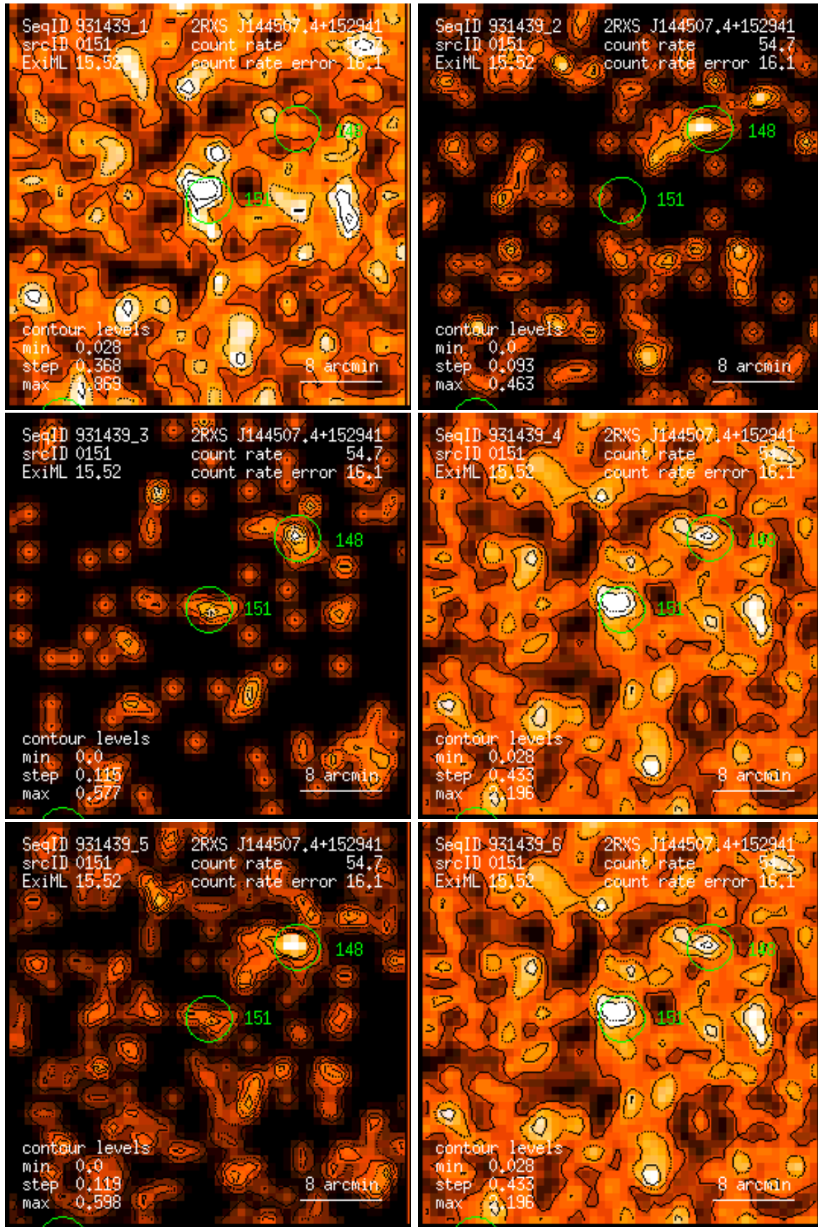
Figure 151: RASS 931439: detection 0151: band rate images, Gaussian filter: (1) PSPC channels 11 – 41, (2) 52 – 90, (3) 91 – 201, (4) 11 – 235, (5) 52 – 201, (6) 11 – 201. Broad band rates in counts/ks. Band rate contour levels in counts/ks/arcmin 2 .
