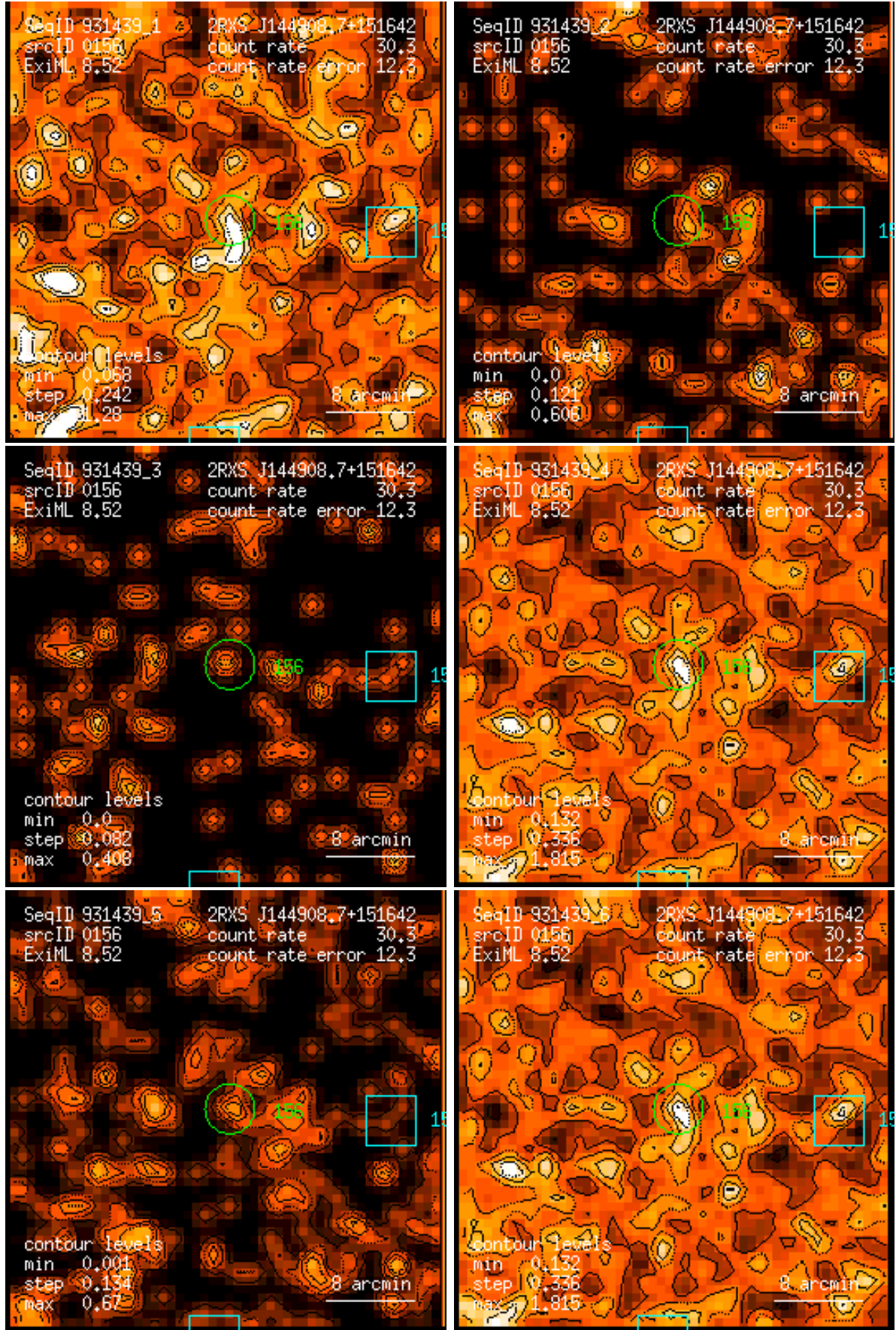
Figure 156: RASS 931439: detection 0156: band rate images, Gaussian filter: (1) PSPC channels 11 – 41, (2) 52 – 90, (3) 91 – 201, (4) 11 – 235, (5) 52 – 201, (6) 11 – 201. Broad band rates in counts/ks. Band rate contour levels in counts/ks/arcmin 2 .
