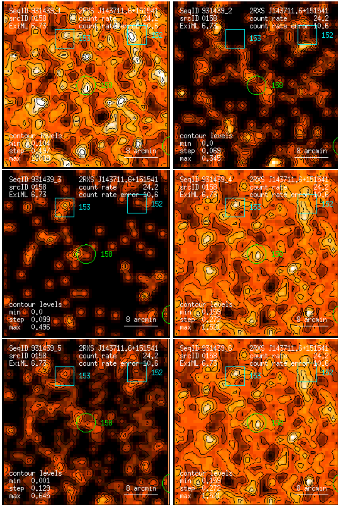
Figure 158: RASS 931439: detection 0158: band rate images, Gaussian filter: (1) PSPC channels 11 – 41, (2) 52 – 90, (3) 91 – 201, (4) 11 – 235, (5) 52 – 201, (6) 11 – 201. Broad band rates in counts/ks. Band rate contour levels in counts/ks/arcmin 2 .
