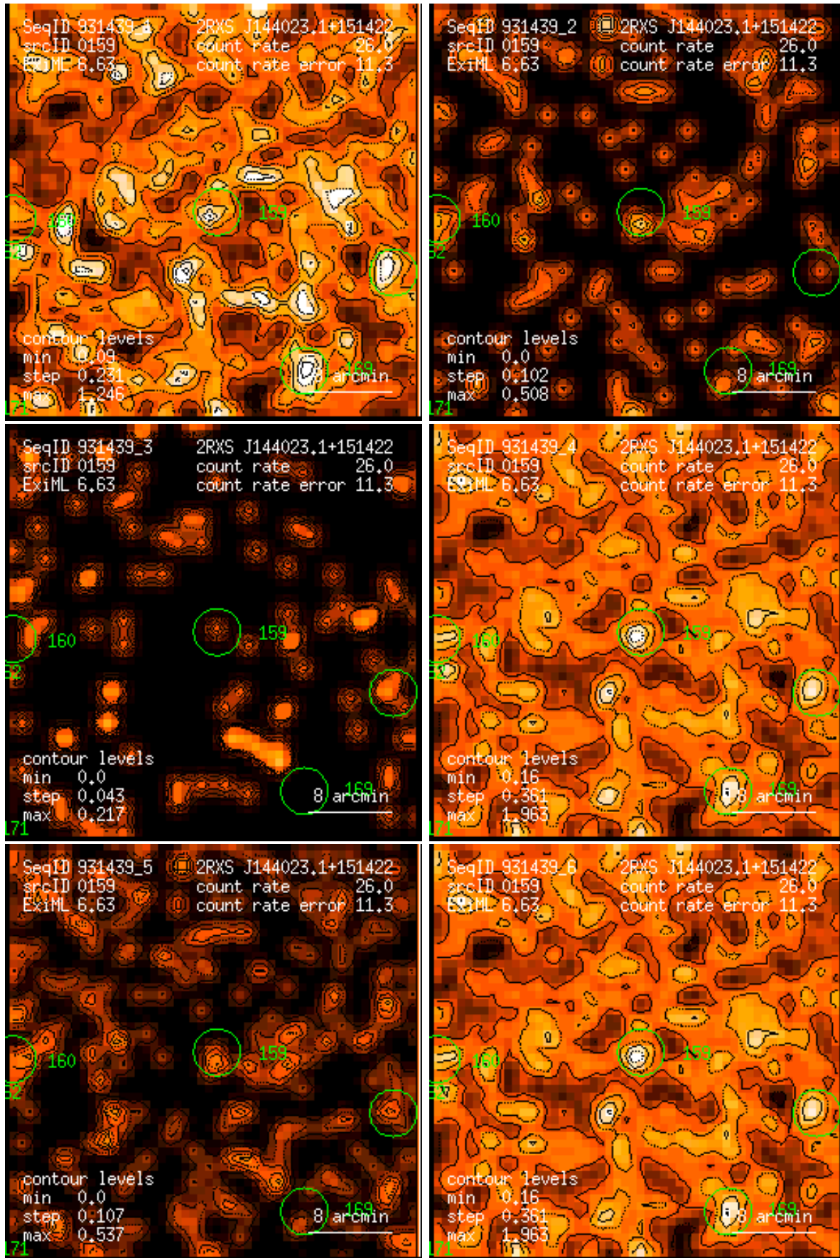
Figure 159: RASS 931439: detection 0159: band rate images, Gaussian filter: (1) PSPC channels 11 – 41, (2) 52 – 90, (3) 91 – 201, (4) 11 – 235, (5) 52 – 201, (6) 11 – 201. Broad band rates in counts/ks. Band rate contour levels in counts/ks/arcmin 2 .
