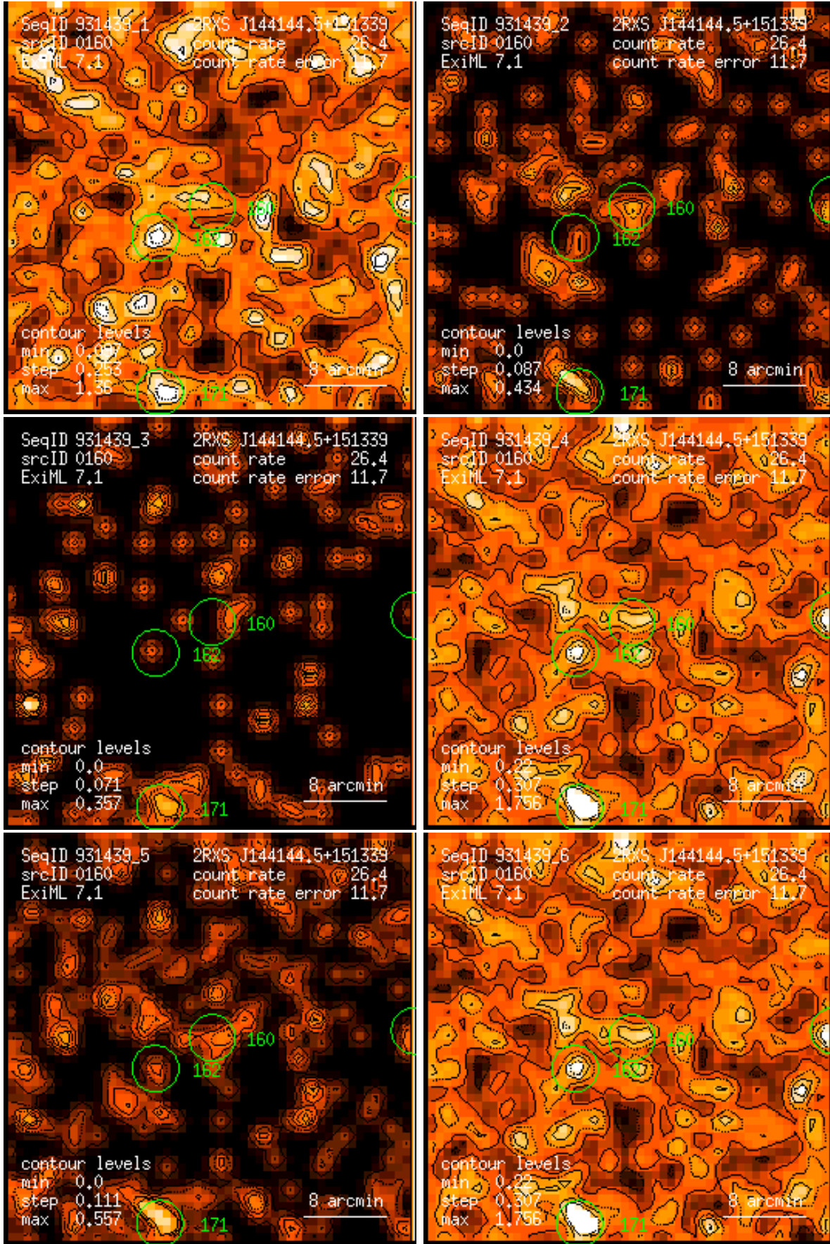
Figure 160: RASS 931439: detection 0160: band rate images, Gaussian filter: (1) PSPC channels 11 – 41, (2) 52 – 90, (3) 91 – 201, (4) 11 – 235, (5) 52 – 201, (6) 11 – 201. Broad band rates in counts/ks. Band rate contour levels in counts/ks/arcmin 2 .
