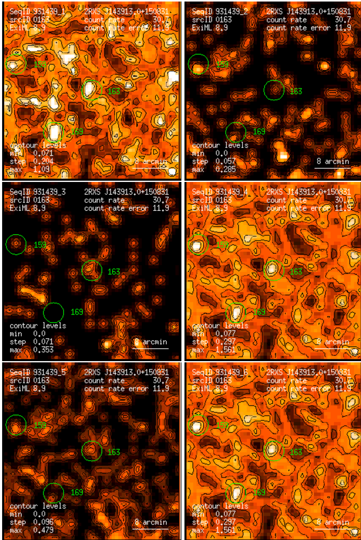
Figure 163: RASS 931439: detection 0163: band rate images, Gaussian filter: (1) PSPC channels 11 – 41, (2) 52 – 90, (3) 91 – 201, (4) 11 – 235, (5) 52 – 201, (6) 11 – 201. Broad band rates in counts/ks. Band rate contour levels in counts/ks/arcmin 2 .
