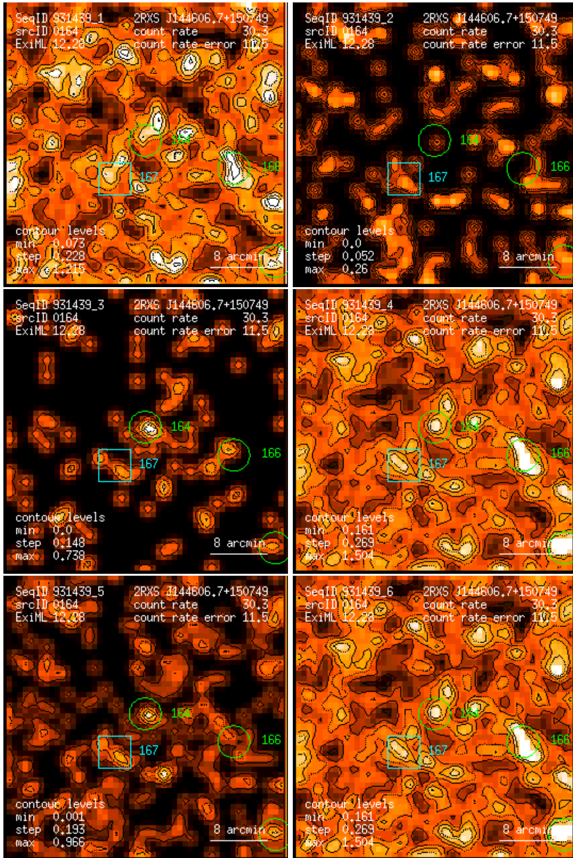
Figure 164: RASS 931439: detection 0164: band rate images, Gaussian filter: (1) PSPC channels 11 – 41, (2) 52 – 90, (3) 91 – 201, (4) 11 – 235, (5) 52 – 201, (6) 11 – 201. Broad band rates in counts/ks. Band rate contour levels in counts/ks/arcmin 2 .
