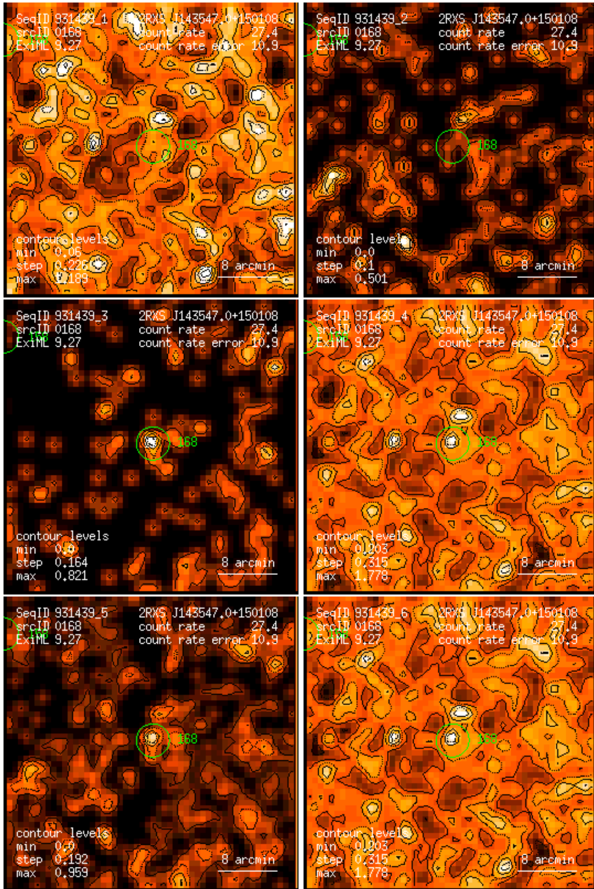
Figure 168: RASS 931439: detection 0168: band rate images, Gaussian filter: (1) PSPC channels 11 – 41, (2) 52 – 90, (3) 91 – 201, (4) 11 – 235, (5) 52 – 201, (6) 11 – 201. Broad band rates in counts/ks. Band rate contour levels in counts/ks/arcmin 2 .
