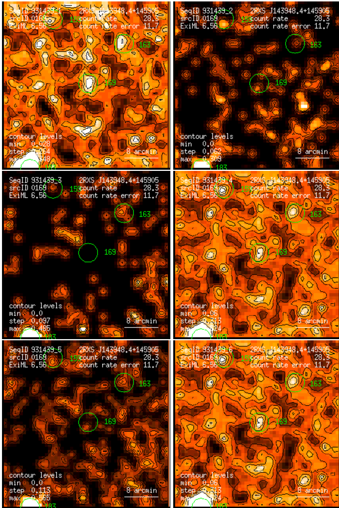
Figure 169: RASS 931439: detection 0169: band rate images, Gaussian filter: (1) PSPC channels 11 – 41, (2) 52 – 90, (3) 91 – 201, (4) 11 – 235, (5) 52 – 201, (6) 11 – 201. Broad band rates in counts/ks. Band rate contour levels in counts/ks/arcmin 2 .
