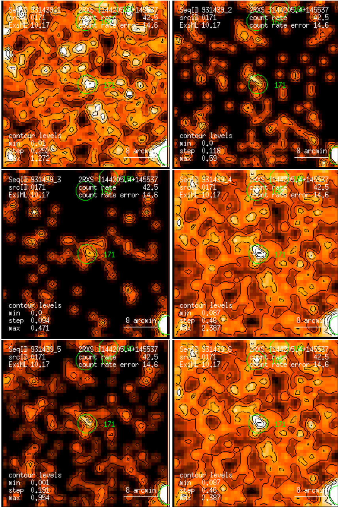
Figure 171: RASS 931439: detection 0171: band rate images, Gaussian filter: (1) PSPC channels 11 – 41, (2) 52 – 90, (3) 91 – 201, (4) 11 – 235, (5) 52 – 201, (6) 11 – 201. Broad band rates in counts/ks. Band rate contour levels in counts/ks/arcmin 2 .
