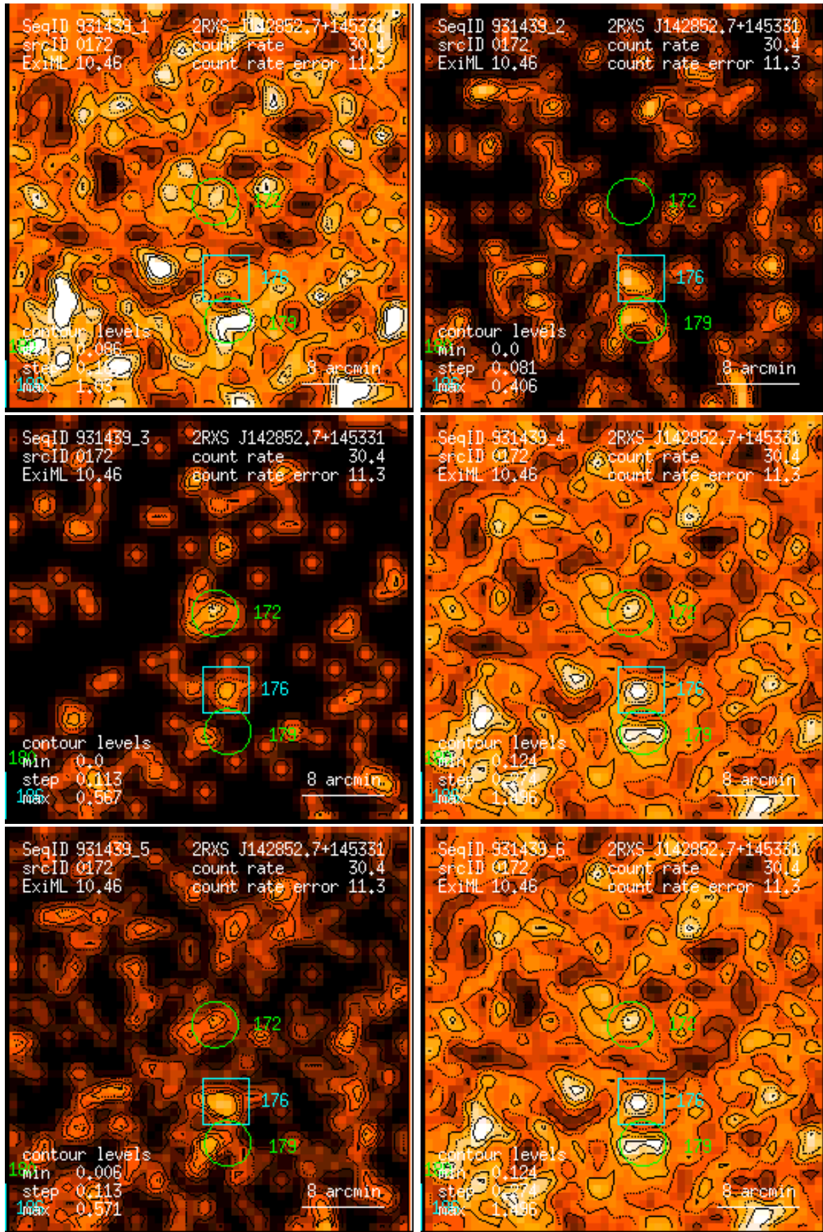
Figure 172: RASS 931439: detection 0172: band rate images, Gaussian filter: (1) PSPC channels 11 – 41, (2) 52 – 90, (3) 91 – 201, (4) 11 – 235, (5) 52 – 201, (6) 11 – 201. Broad band rates in counts/ks. Band rate contour levels in counts/ks/arcmin 2 .
