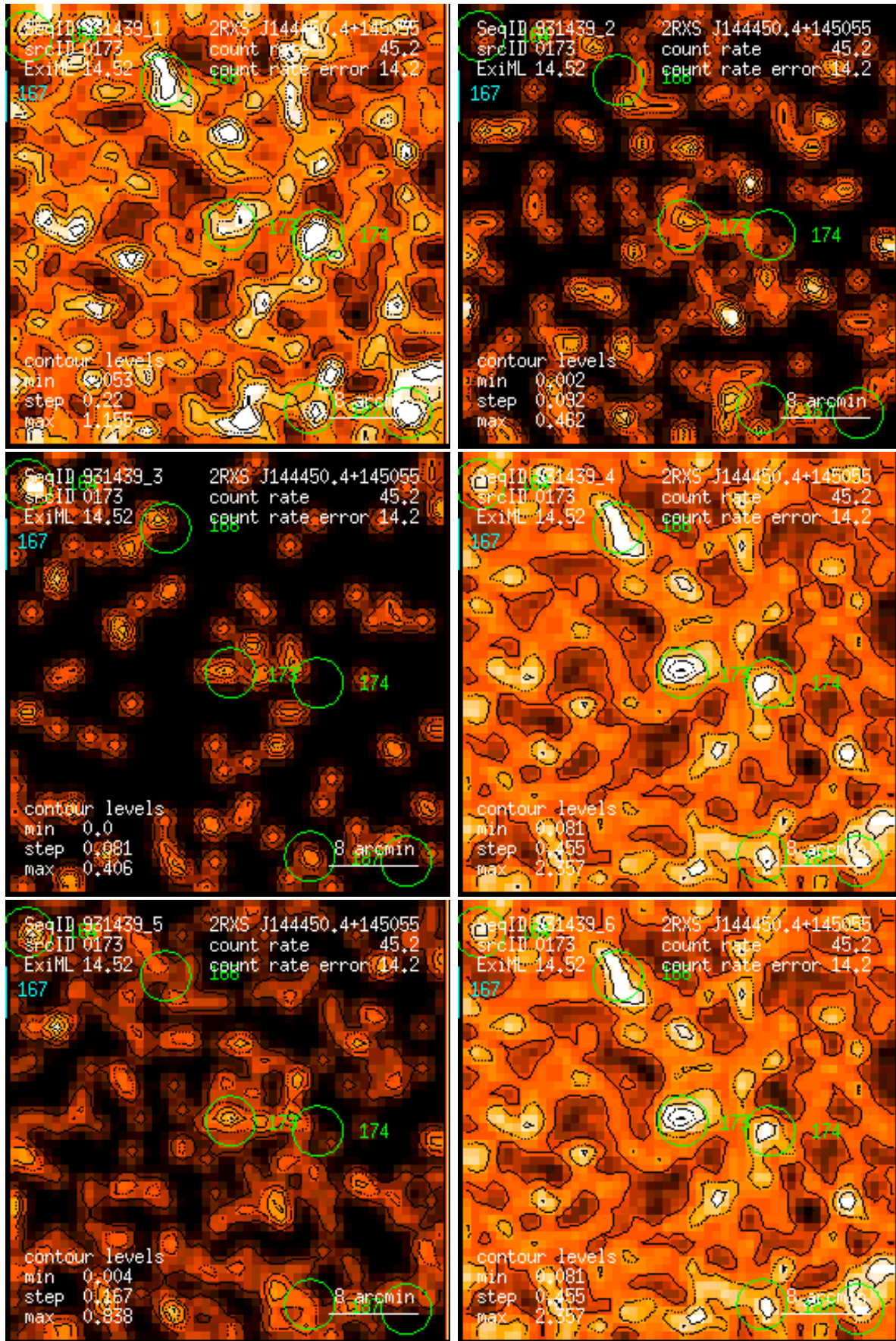
Figure 173: RASS 931439: detection 0173: band rate images, Gaussian filter: (1) PSPC channels 11 – 41, (2) 52 – 90, (3) 91 – 201, (4) 11 – 235, (5) 52 – 201, (6) 11 – 201. Broad band rates in counts/ks. Band rate contour levels in counts/ks/arcmin 2 .
