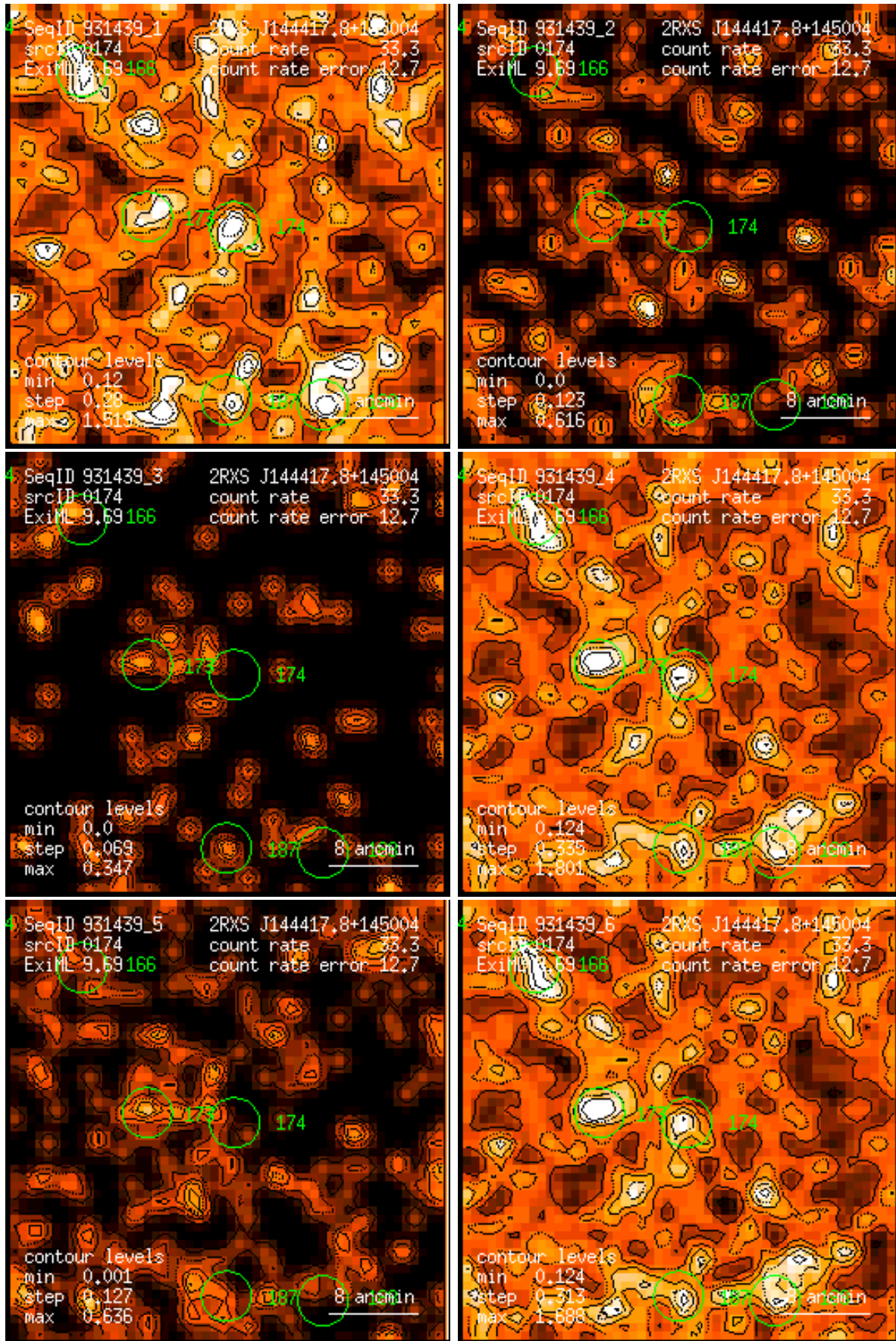
Figure 174: RASS 931439: detection 0174: band rate images, Gaussian filter: (1) PSPC channels 11 – 41, (2) 52 – 90, (3) 91 – 201, (4) 11 – 235, (5) 52 – 201, (6) 11 – 201. Broad band rates in counts/ks. Band rate contour levels in counts/ks/arcmin 2 .
