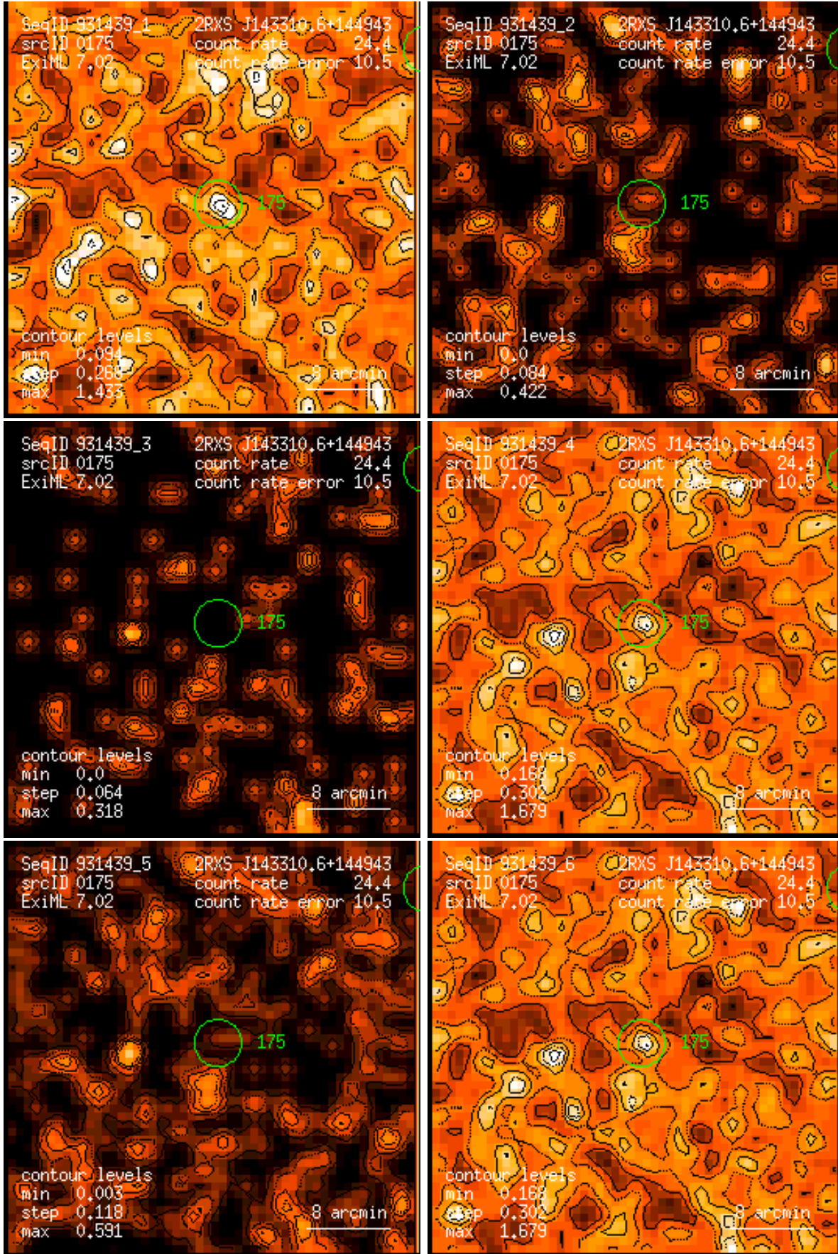
Figure 175: RASS 931439: detection 0175: band rate images, Gaussian filter: (1) PSPC channels 11 – 41, (2) 52 – 90, (3) 91 – 201, (4) 11 – 235, (5) 52 – 201, (6) 11 – 201. Broad band rates in counts/ks. Band rate contour levels in counts/ks/arcmin 2 .
