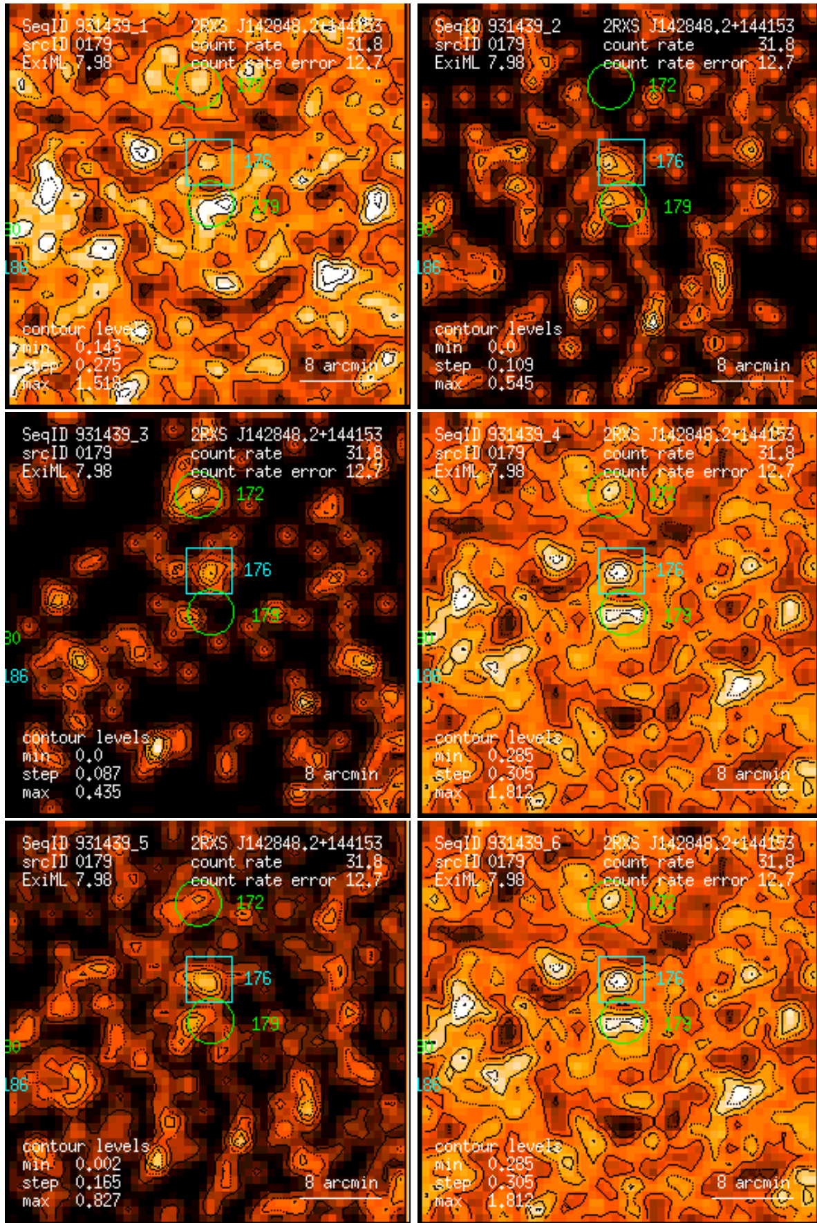
Figure 179: RASS 931439: detection 0179: band rate images, Gaussian filter: (1) PSPC channels 11 – 41, (2) 52 – 90, (3) 91 – 201, (4) 11 – 235, (5) 52 – 201, (6) 11 – 201. Broad band rates in counts/ks. Band rate contour levels in counts/ks/arcmin 2 .
