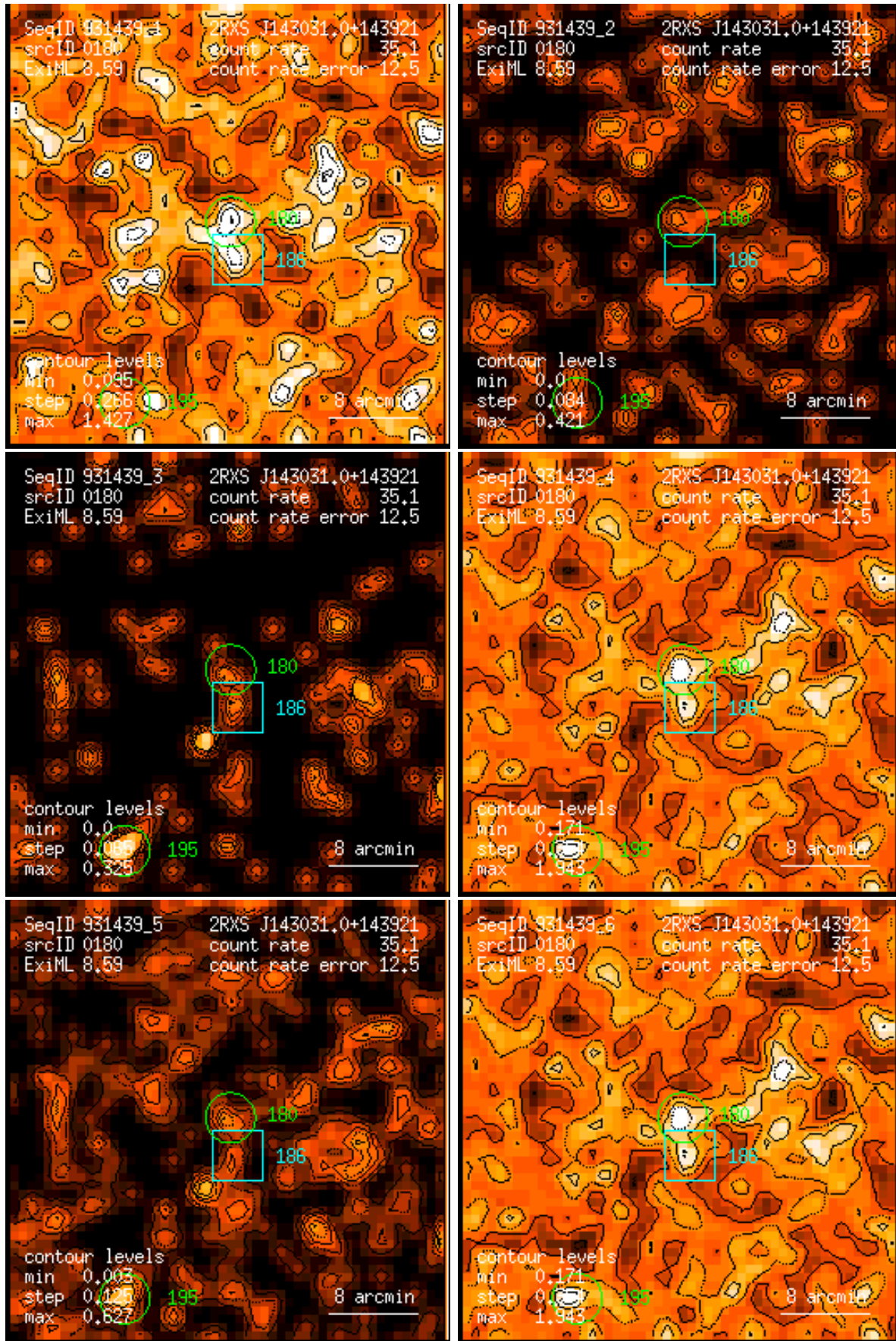
Figure 180: RASS 931439: detection 0180: band rate images, Gaussian filter: (1) PSPC channels 11 – 41, (2) 52 – 90, (3) 91 – 201, (4) 11 – 235, (5) 52 – 201, (6) 11 – 201. Broad band rates in counts/ks. Band rate contour levels in counts/ks/arcmin 2 .
