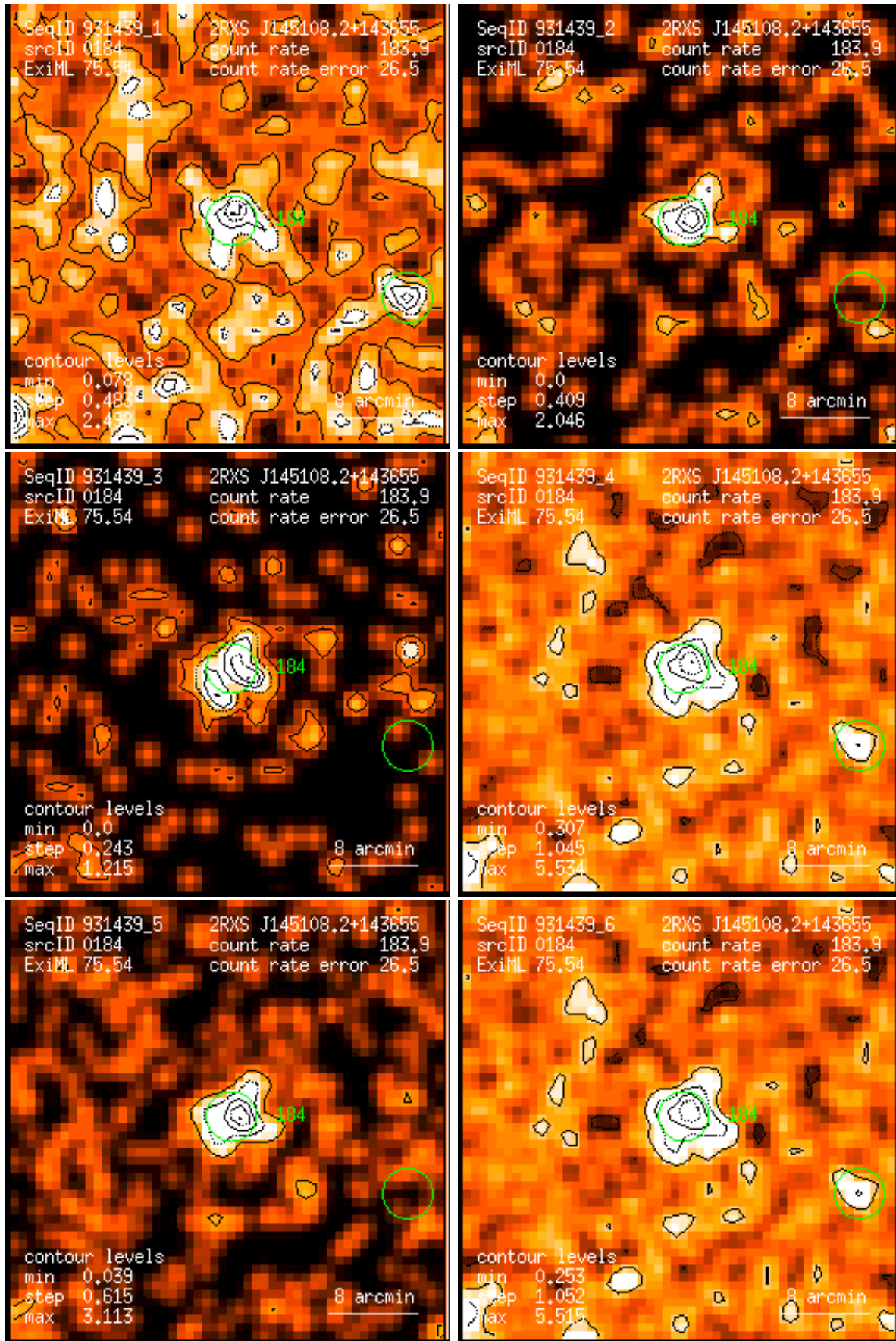
Figure 184: RASS 931439: detection 0184: band rate images, Gaussian filter: (1) PSPC channels 11 – 41, (2) 52 – 90, (3) 91 – 201, (4) 11 – 235, (5) 52 – 201, (6) 11 – 201. Broad band rates in counts/ks. Band rate contour levels in counts/ks/arcmin 2 .
