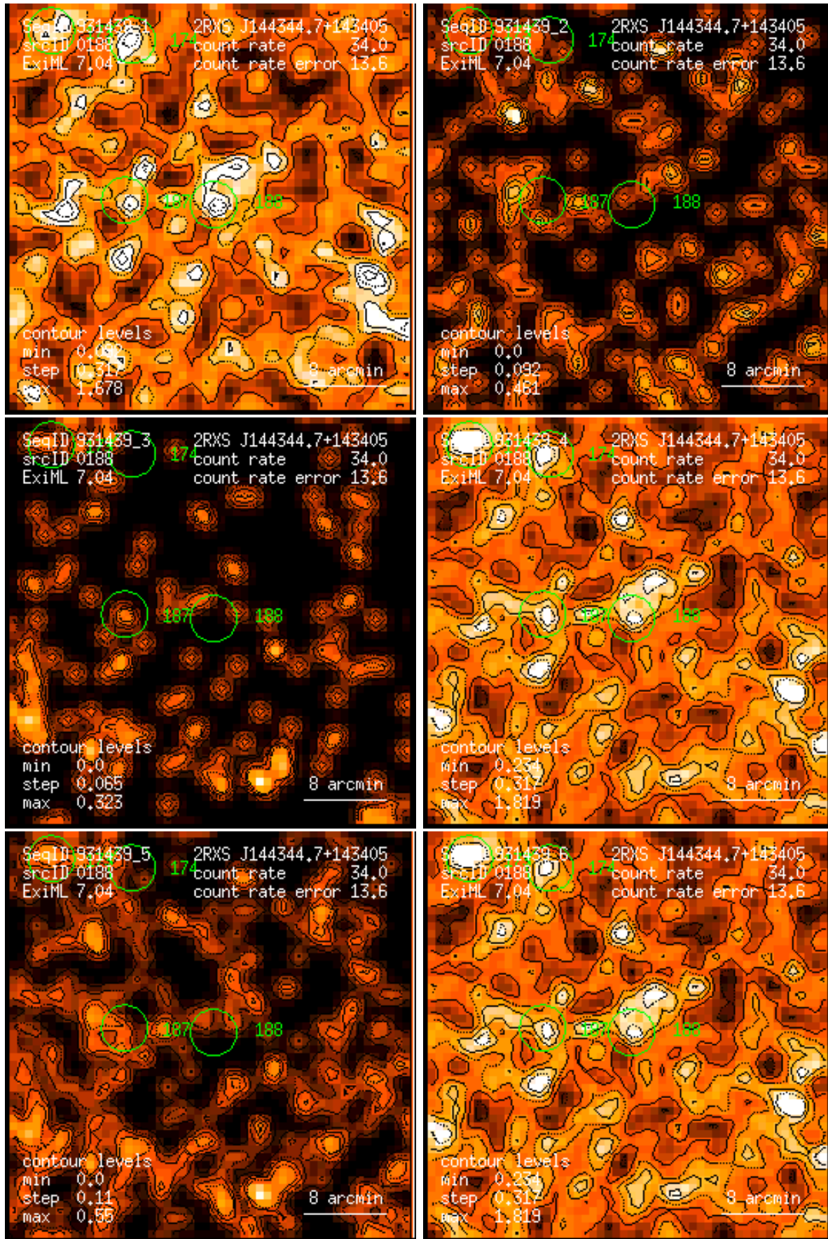
Figure 188: RASS 931439: detection 0188: band rate images, Gaussian filter: (1) PSPC channels 11 – 41, (2) 52 – 90, (3) 91 – 201, (4) 11 – 235, (5) 52 – 201, (6) 11 – 201. Broad band rates in counts/ks. Band rate contour levels in counts/ks/arcmin 2 .
