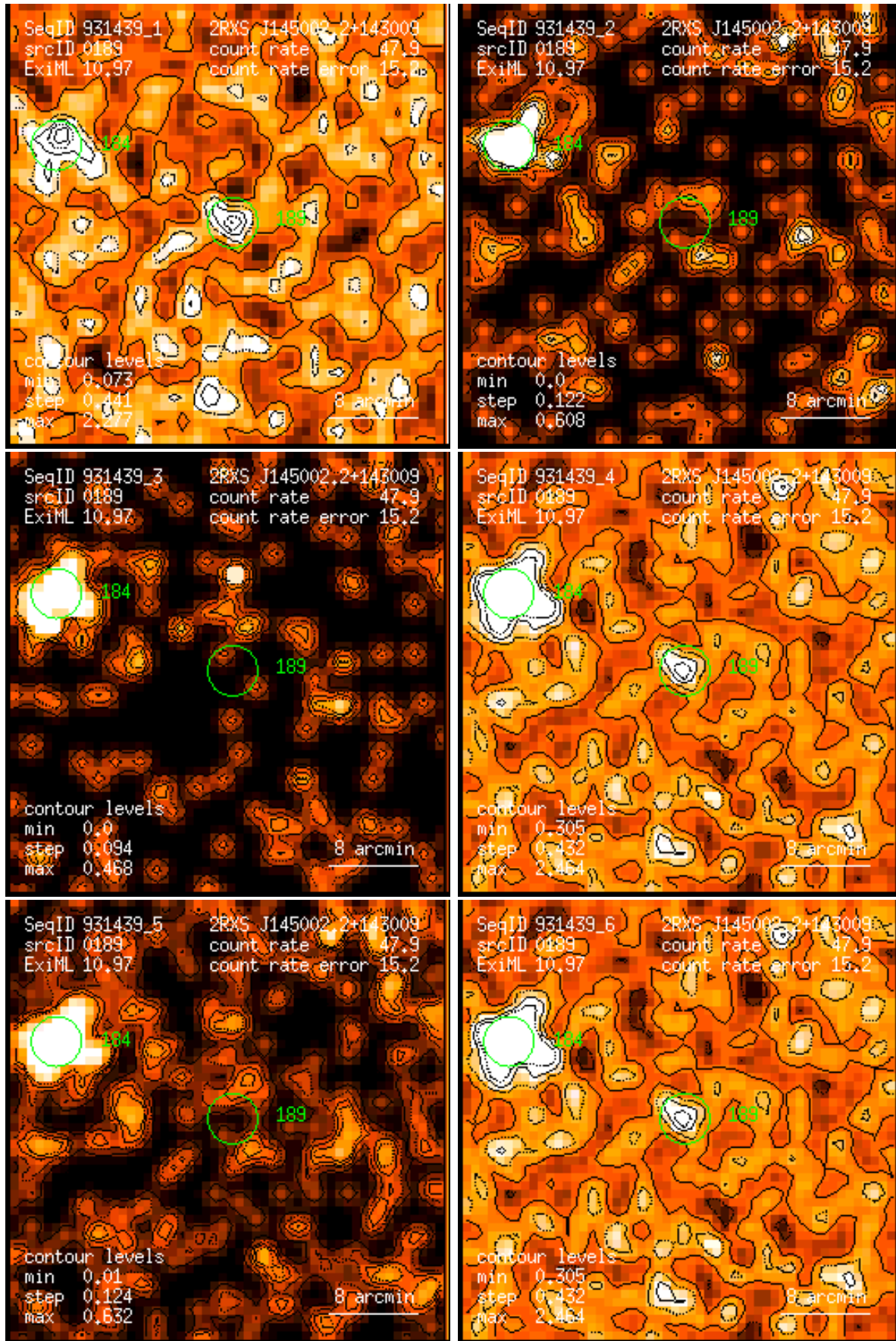
Figure 189: RASS 931439: detection 0189: band rate images, Gaussian filter: (1) PSPC channels 11 – 41, (2) 52 – 90, (3) 91 – 201, (4) 11 – 235, (5) 52 – 201, (6) 11 – 201. Broad band rates in counts/ks. Band rate contour levels in counts/ks/arcmin 2 .
