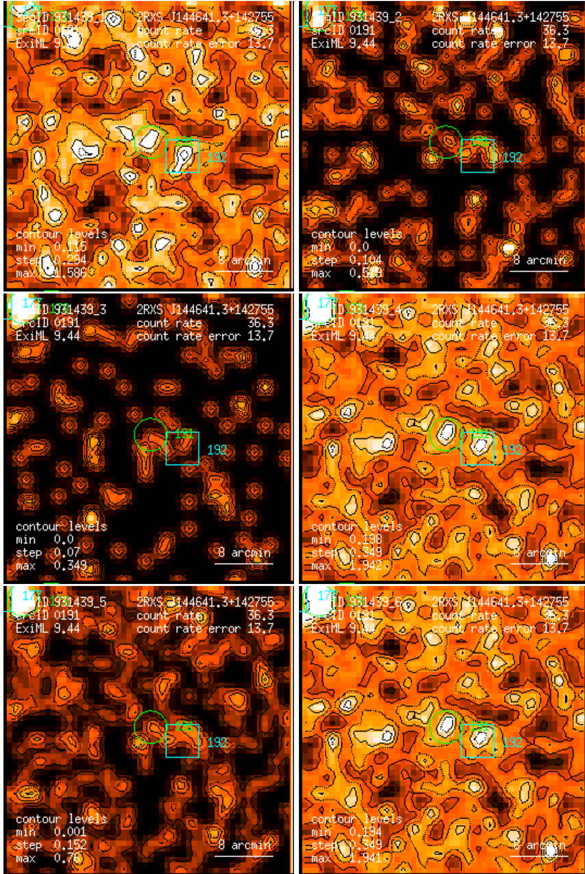
Figure 191: RASS 931439: detection 0191: band rate images, Gaussian filter: (1) PSPC channels 11 – 41, (2) 52 – 90, (3) 91 – 201, (4) 11 – 235, (5) 52 – 201, (6) 11 – 201. Broad band rates in counts/ks. Band rate contour levels in counts/ks/arcmin 2 .
