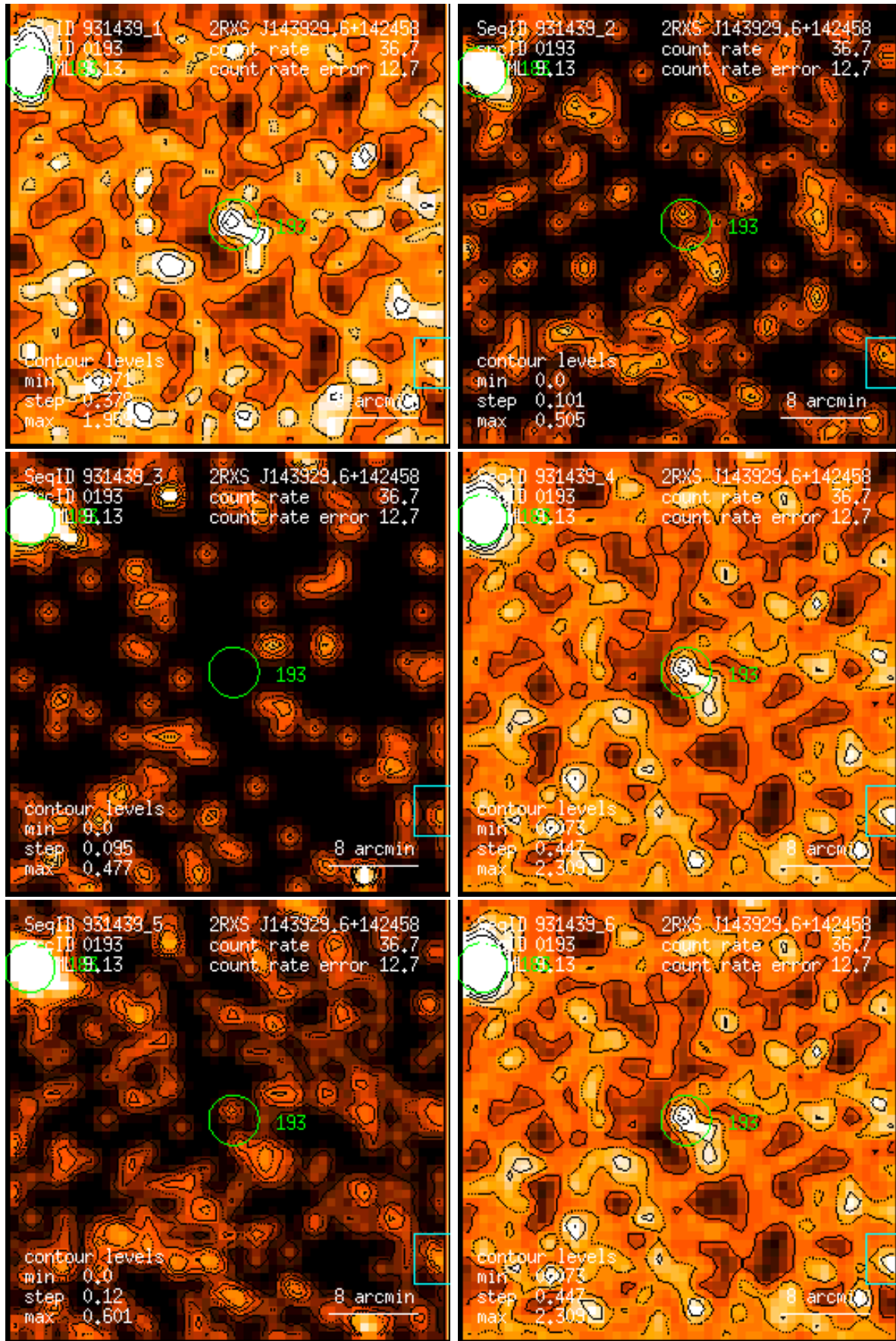
Figure 193: RASS 931439: detection 0193: band rate images, Gaussian filter: (1) PSPC channels 11 – 41, (2) 52 – 90, (3) 91 – 201, (4) 11 – 235, (5) 52 – 201, (6) 11 – 201. Broad band rates in counts/ks. Band rate contour levels in counts/ks/arcmin 2 .
