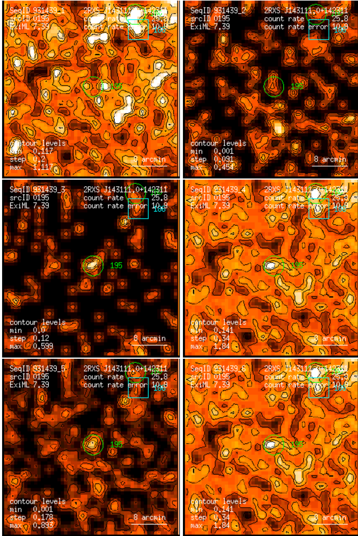
Figure 195: RASS 931439: detection 0195: band rate images, Gaussian filter: (1) PSPC channels 11 – 41, (2) 52 – 90, (3) 91 – 201, (4) 11 – 235, (5) 52 – 201, (6) 11 – 201. Broad band rates in counts/ks. Band rate contour levels in counts/ks/arcmin 2 .
