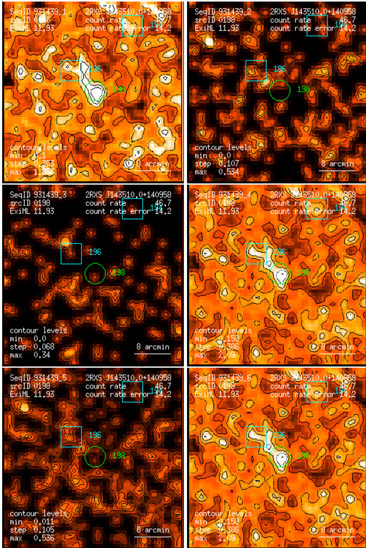
Figure 198: RASS 931439: detection 0198: band rate images, Gaussian filter: (1) PSPC channels 11 – 41, (2) 52 – 90, (3) 91 – 201, (4) 11 – 235, (5) 52 – 201, (6) 11 – 201. Broad band rates in counts/ks. Band rate contour levels in counts/ks/arcmin 2 .
