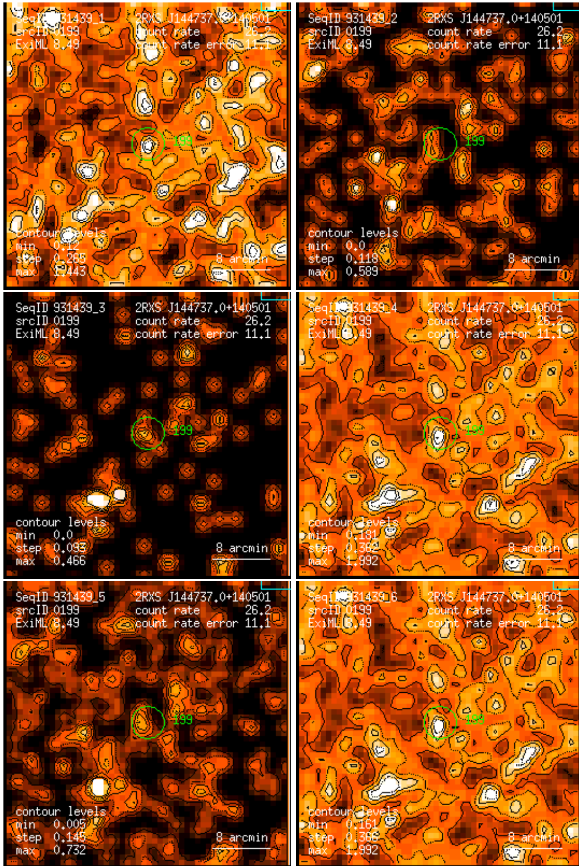
Figure 199: RASS 931439: detection 0199: band rate images, Gaussian filter: (1) PSPC channels 11 – 41, (2) 52 – 90, (3) 91 – 201, (4) 11 – 235, (5) 52 – 201, (6) 11 – 201. Broad band rates in counts/ks. Band rate contour levels in counts/ks/arcmin 2 .
