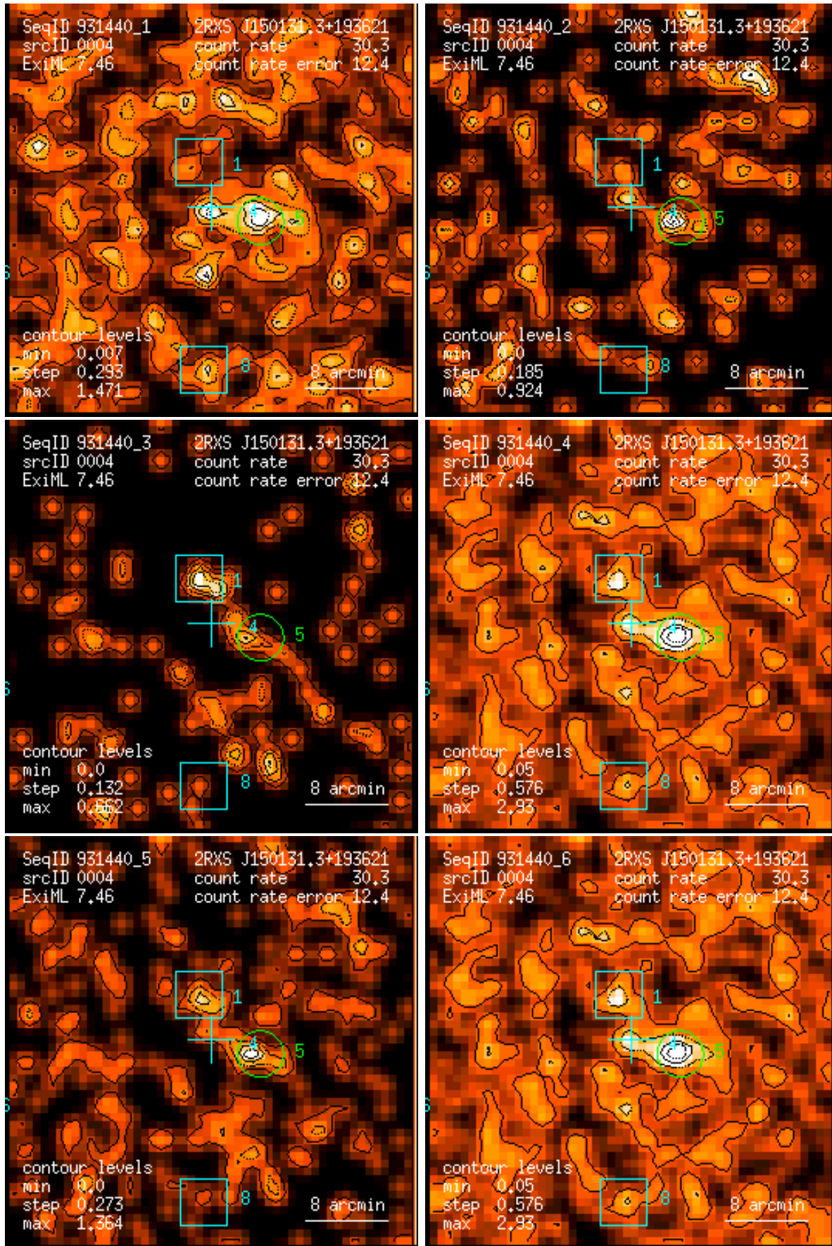
Figure 4: RASS 931440: detection 0004: band rate images, Gaussian filter: (1) PSPC channels 11 – 41, (2) 52 – 90, (3) 91 – 201, (4) 11 – 235, (5) 52 – 201, (6) 11 – 201. Broad band rates in counts/ks. Band rate contour levels in counts/ks/arcmin 2 .
