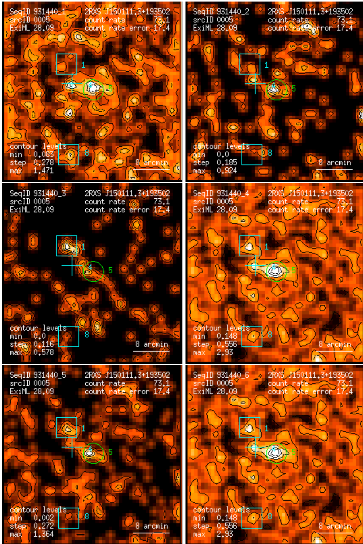
Figure 5: RASS 931440: detection 0005: band rate images, Gaussian filter: (1) PSPC channels 11 – 41, (2) 52 – 90, (3) 91 – 201, (4) 11 – 235, (5) 52 – 201, (6) 11 – 201. Broad band rates in counts/ks. Band rate contour levels in counts/ks/arcmin 2 .
