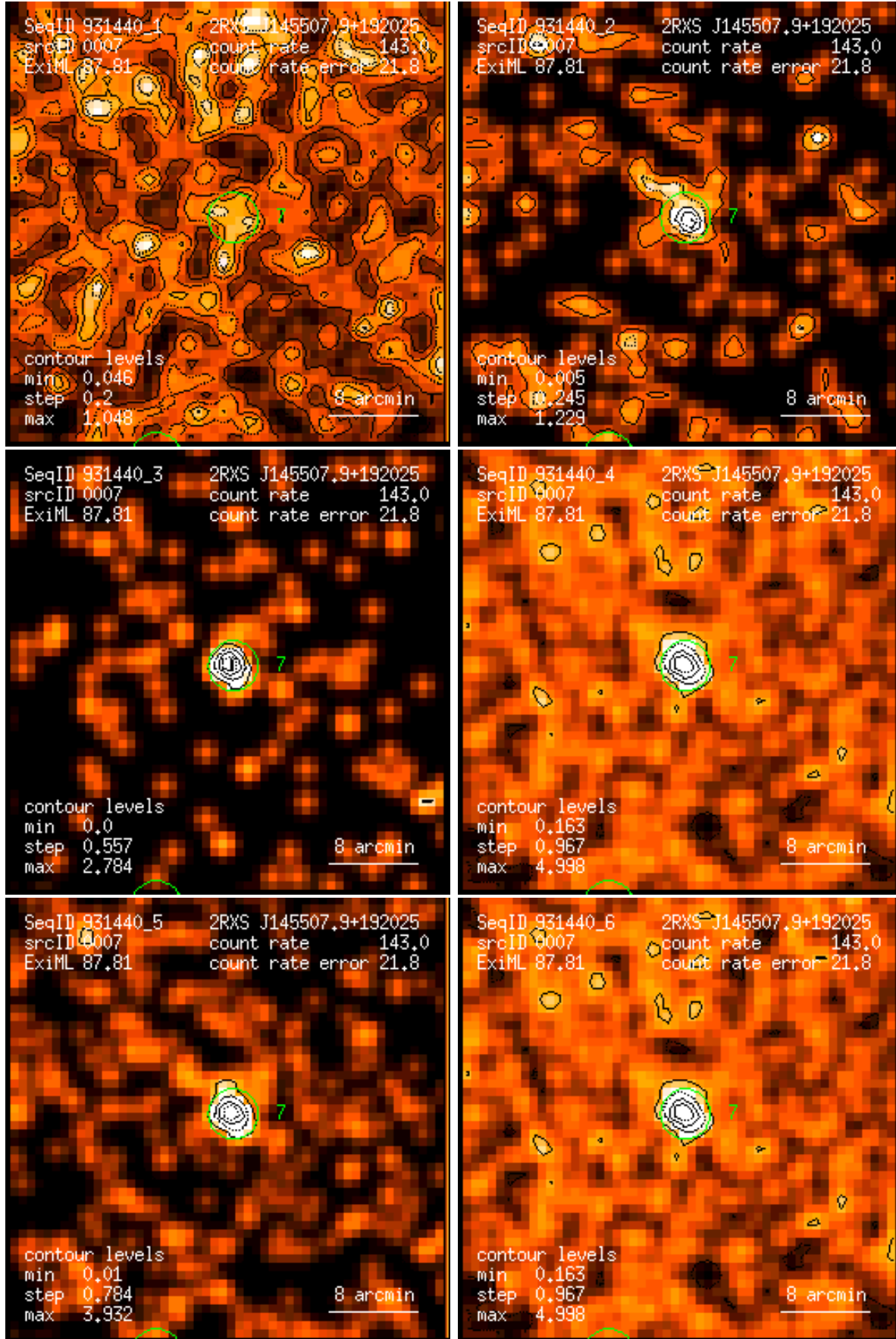
Figure 7: RASS 931440: detection 0007: band rate images, Gaussian filter: (1) PSPC channels 11 – 41, (2) 52 – 90, (3) 91 – 201, (4) 11 – 235, (5) 52 – 201, (6) 11 – 201. Broad band rates in counts/ks. Band rate contour levels in counts/ks/arcmin 2 .
