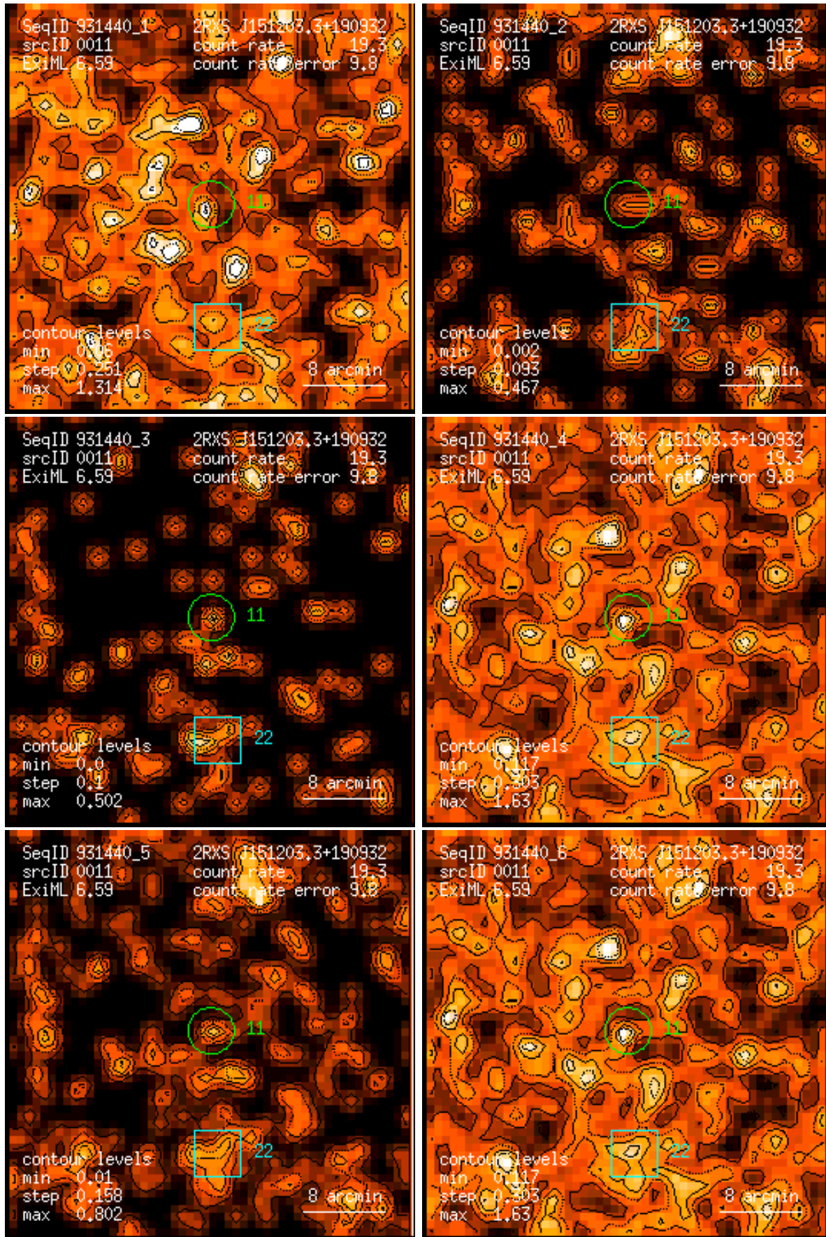
Figure 11: RASS 931440: detection 0011: band rate images, Gaussian filter: (1) PSPC channels 11 – 41, (2) 52 – 90, (3) 91 – 201, (4) 11 – 235, (5) 52 – 201, (6) 11 – 201. Broad band rates in counts/ks. Band rate contour levels in counts/ks/arcmin 2 .
