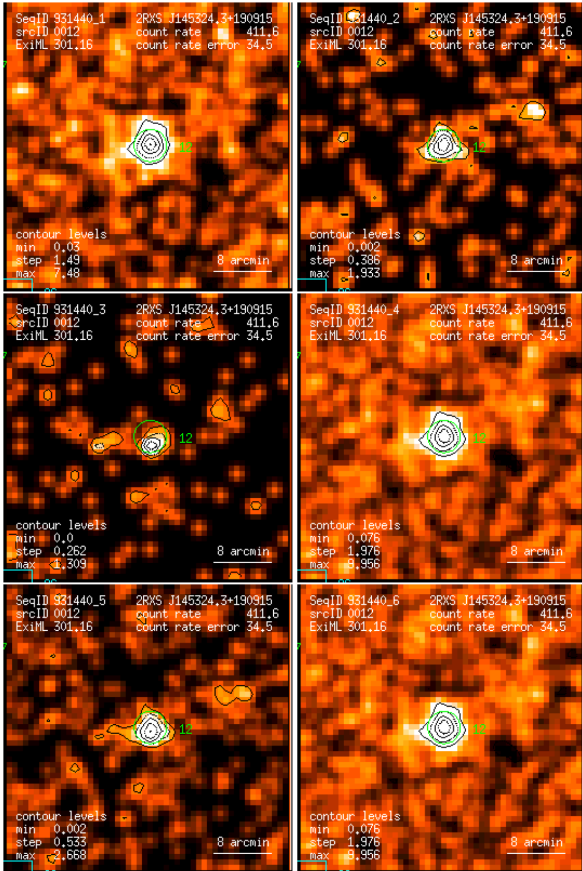
Figure 12: RASS 931440: detection 0012: band rate images, Gaussian filter: (1) PSPC channels 11 – 41, (2) 52 – 90, (3) 91 – 201, (4) 11 – 235, (5) 52 – 201, (6) 11 – 201. Broad band rates in counts/ks. Band rate contour levels in counts/ks/arcmin 2 .
