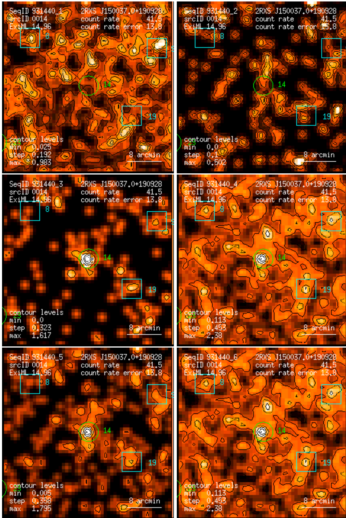
Figure 14: RASS 931440: detection 0014: band rate images, Gaussian filter: (1) PSPC channels 11 – 41, (2) 52 – 90, (3) 91 – 201, (4) 11 – 235, (5) 52 – 201, (6) 11 – 201. Broad band rates in counts/ks. Band rate contour levels in counts/ks/arcmin 2 .
