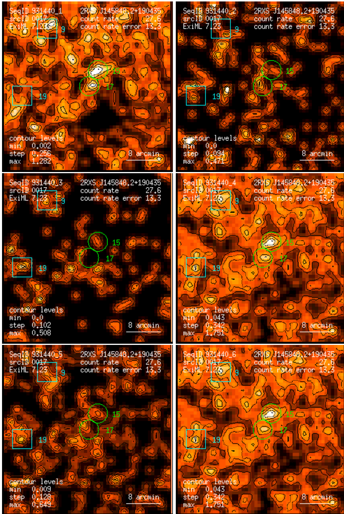
Figure 17: RASS 931440: detection 0017: band rate images, Gaussian filter: (1) PSPC channels 11 – 41, (2) 52 – 90, (3) 91 – 201, (4) 11 – 235, (5) 52 – 201, (6) 11 – 201. Broad band rates in counts/ks. Band rate contour levels in counts/ks/arcmin 2 .
