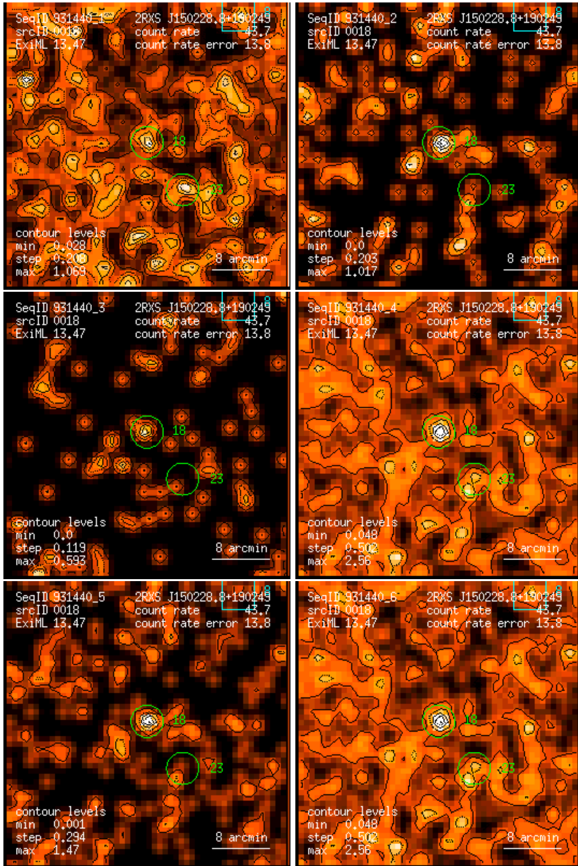
Figure 18: RASS 931440: detection 0018: band rate images, Gaussian filter: (1) PSPC channels 11 – 41, (2) 52 – 90, (3) 91 – 201, (4) 11 – 235, (5) 52 – 201, (6) 11 – 201. Broad band rates in counts/ks. Band rate contour levels in counts/ks/arcmin 2 .
