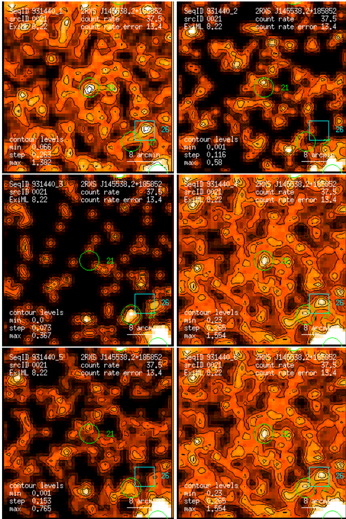
Figure 21: RASS 931440: detection 0021: band rate images, Gaussian filter: (1) PSPC channels 11 – 41, (2) 52 – 90, (3) 91 – 201, (4) 11 – 235, (5) 52 – 201, (6) 11 – 201. Broad band rates in counts/ks. Band rate contour levels in counts/ks/arcmin 2 .
