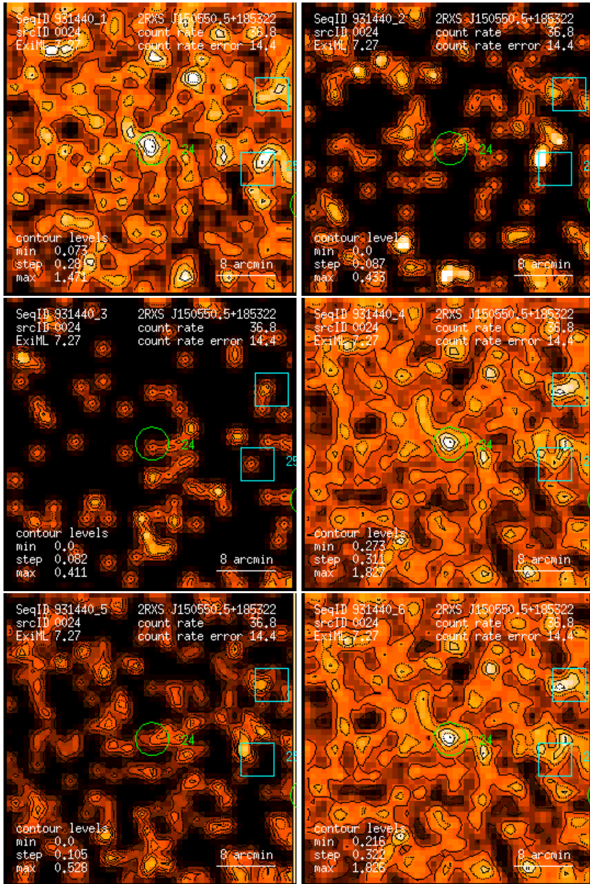
Figure 24: RASS 931440: detection 0024: band rate images, Gaussian filter: (1) PSPC channels 11 – 41, (2) 52 – 90, (3) 91 – 201, (4) 11 – 235, (5) 52 – 201, (6) 11 – 201. Broad band rates in counts/ks. Band rate contour levels in counts/ks/arcmin 2 .
