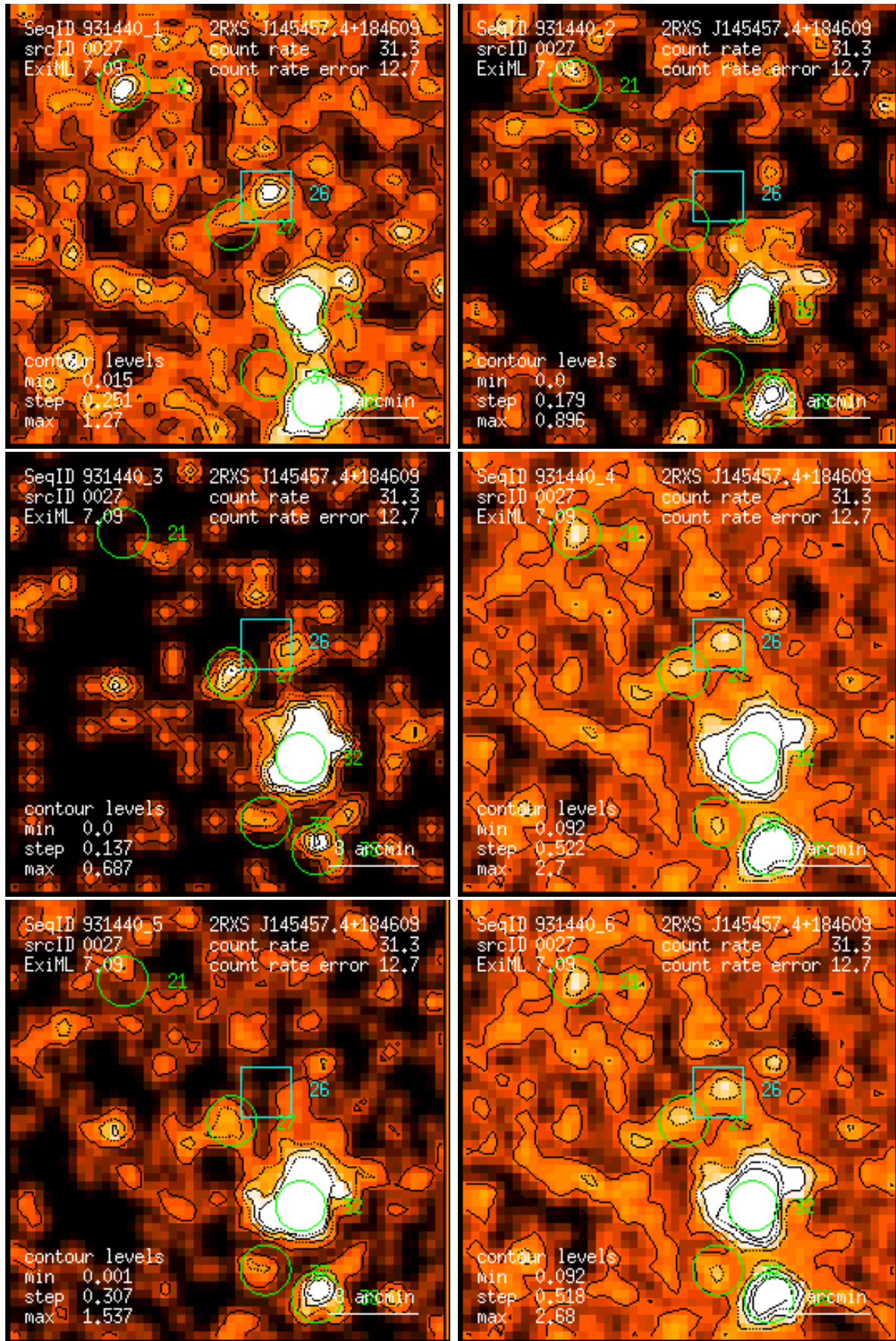
Figure 27: RASS 931440: detection 0027: band rate images, Gaussian filter: (1) PSPC channels 11 – 41, (2) 52 – 90, (3) 91 – 201, (4) 11 – 235, (5) 52 – 201, (6) 11 – 201. Broad band rates in counts/ks. Band rate contour levels in counts/ks/arcmin 2 .
