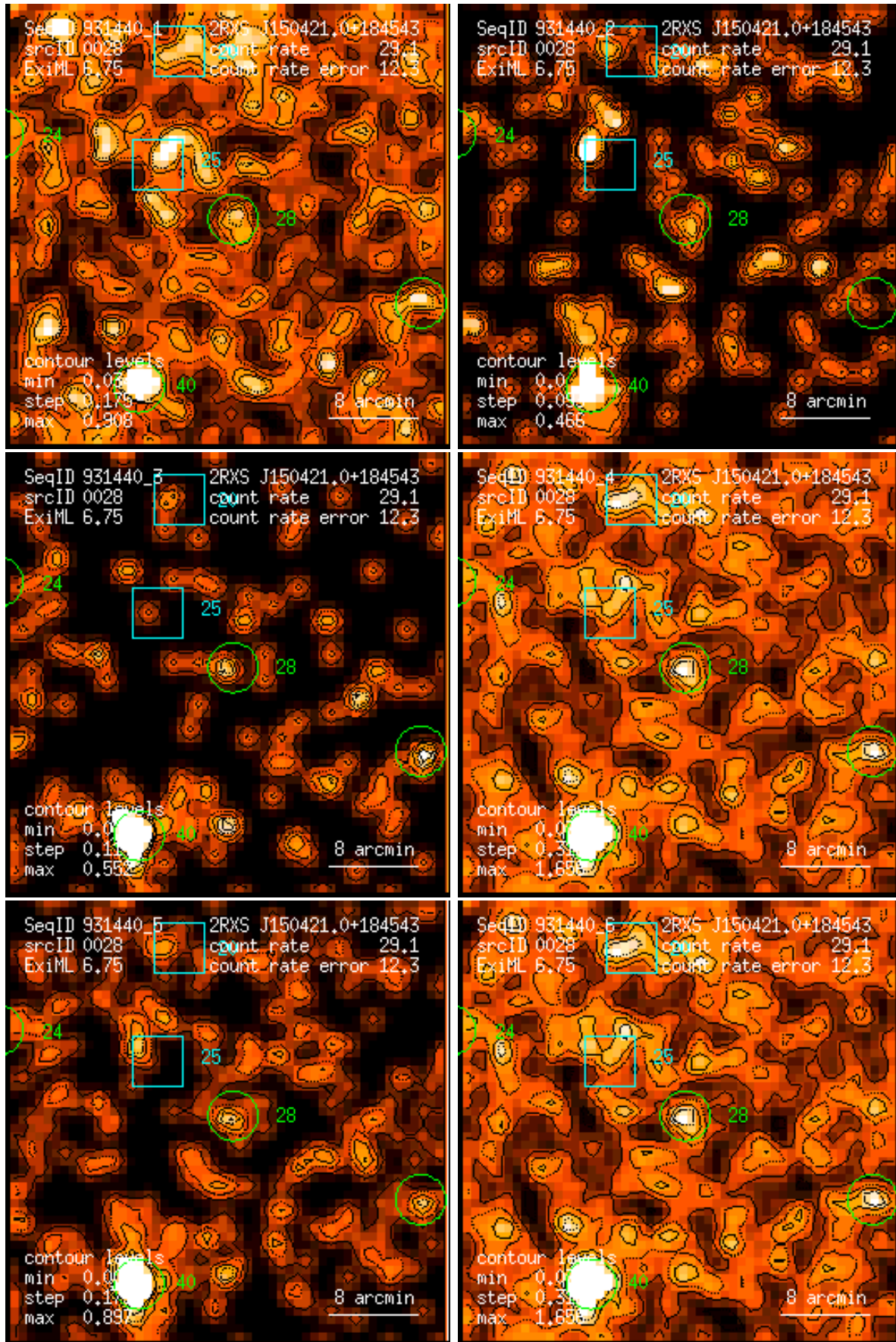
Figure 28: RASS 931440: detection 0028: band rate images, Gaussian filter: (1) PSPC channels 11 – 41, (2) 52 – 90, (3) 91 – 201, (4) 11 – 235, (5) 52 – 201, (6) 11 – 201. Broad band rates in counts/ks. Band rate contour levels in counts/ks/arcmin 2 .
