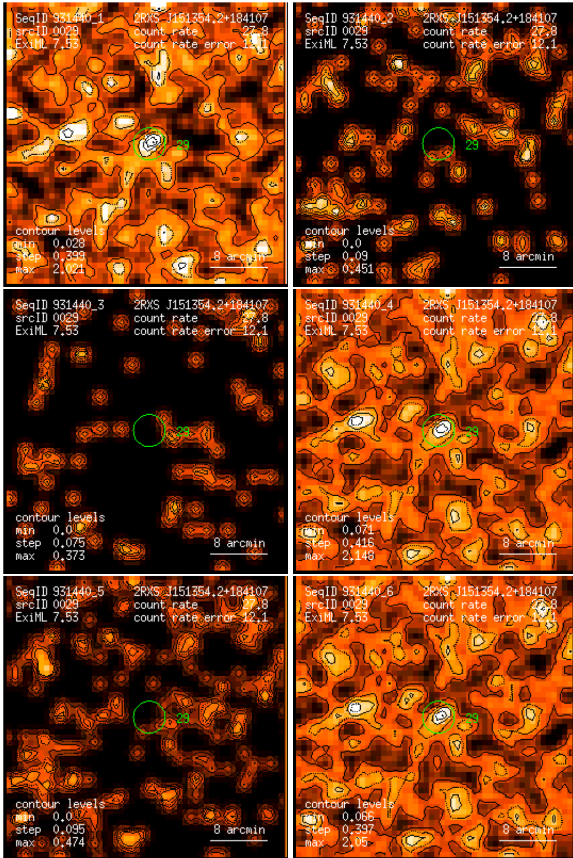
Figure 29: RASS 931440: detection 0029: band rate images, Gaussian filter: (1) PSPC channels 11 – 41, (2) 52 – 90, (3) 91 – 201, (4) 11 – 235, (5) 52 – 201, (6) 11 – 201. Broad band rates in counts/ks. Band rate contour levels in counts/ks/arcmin 2 .
