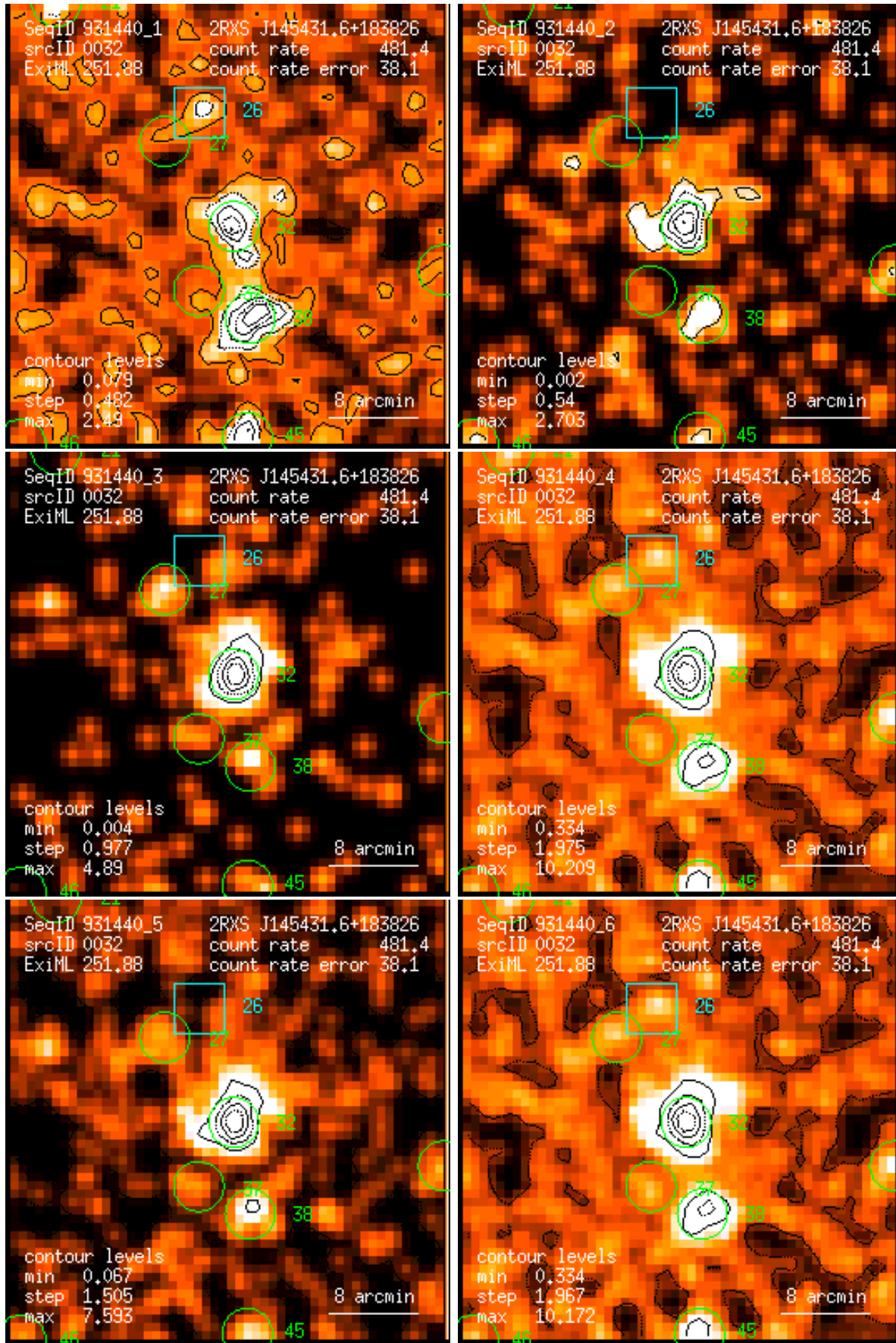
Figure 32: RASS 931440: detection 0032: band rate images, Gaussian filter: (1) PSPC channels 11 – 41, (2) 52 – 90, (3) 91 – 201, (4) 11 – 235, (5) 52 – 201, (6) 11 – 201. Broad band rates in counts/ks. Band rate contour levels in counts/ks/arcmin 2 .
