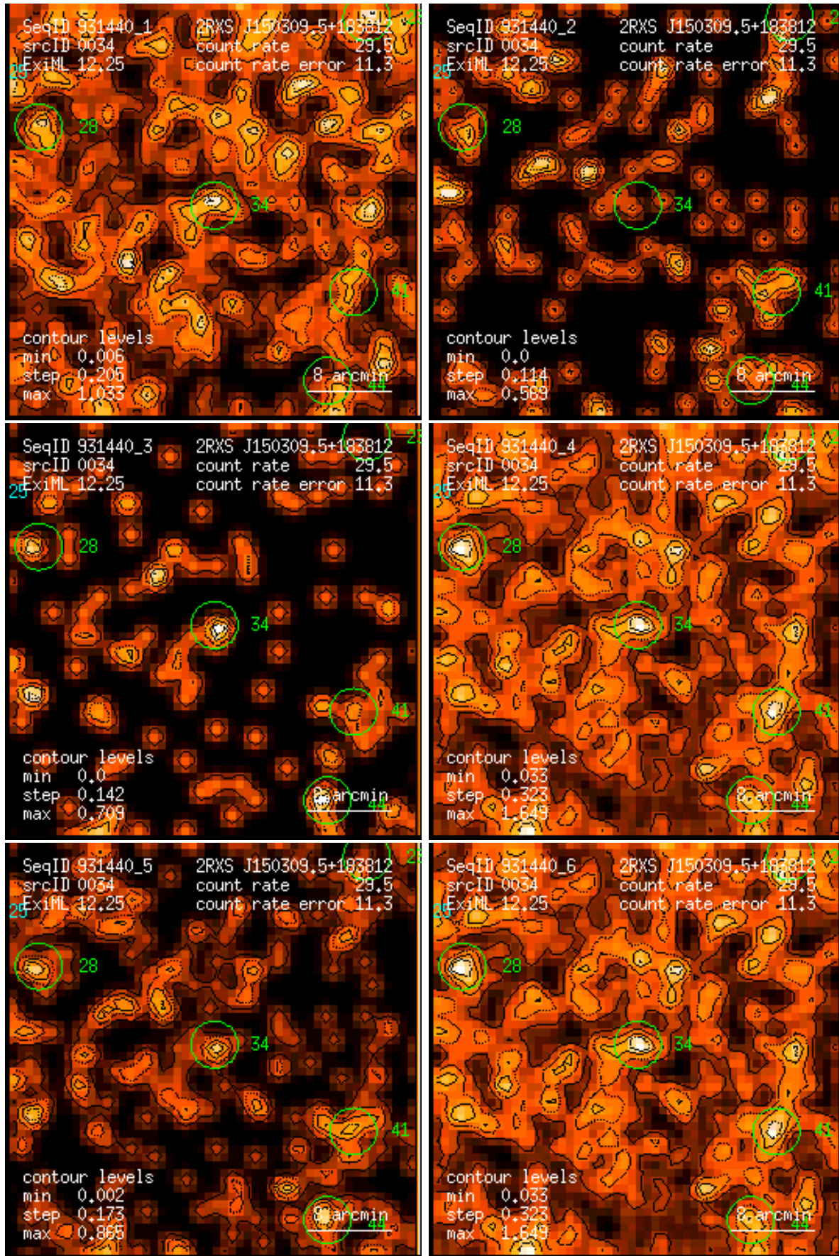
Figure 34: RASS 931440: detection 0034: band rate images, Gaussian filter: (1) PSPC channels 11 – 41, (2) 52 – 90, (3) 91 – 201, (4) 11 – 235, (5) 52 – 201, (6) 11 – 201. Broad band rates in counts/ks. Band rate contour levels in counts/ks/arcmin 2 .
