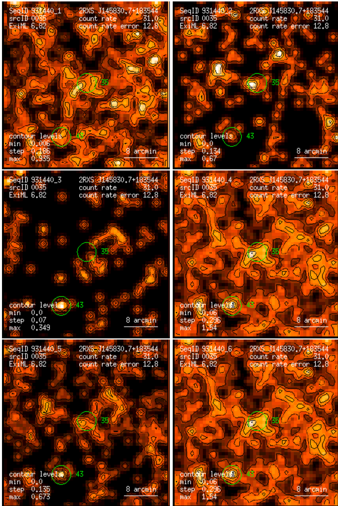
Figure 35: RASS 931440: detection 0035: band rate images, Gaussian filter: (1) PSPC channels 11 – 41, (2) 52 – 90, (3) 91 – 201, (4) 11 – 235, (5) 52 – 201, (6) 11 – 201. Broad band rates in counts/ks. Band rate contour levels in counts/ks/arcmin 2 .
