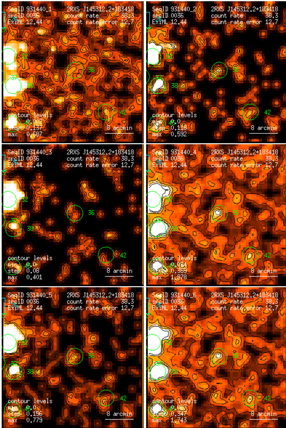
Figure 36: RASS 931440: detection 0036: band rate images, Gaussian filter: (1) PSPC channels 11 – 41, (2) 52 – 90, (3) 91 – 201, (4) 11 – 235, (5) 52 – 201, (6) 11 – 201. Broad band rates in counts/ks. Band rate contour levels in counts/ks/arcmin 2 .
