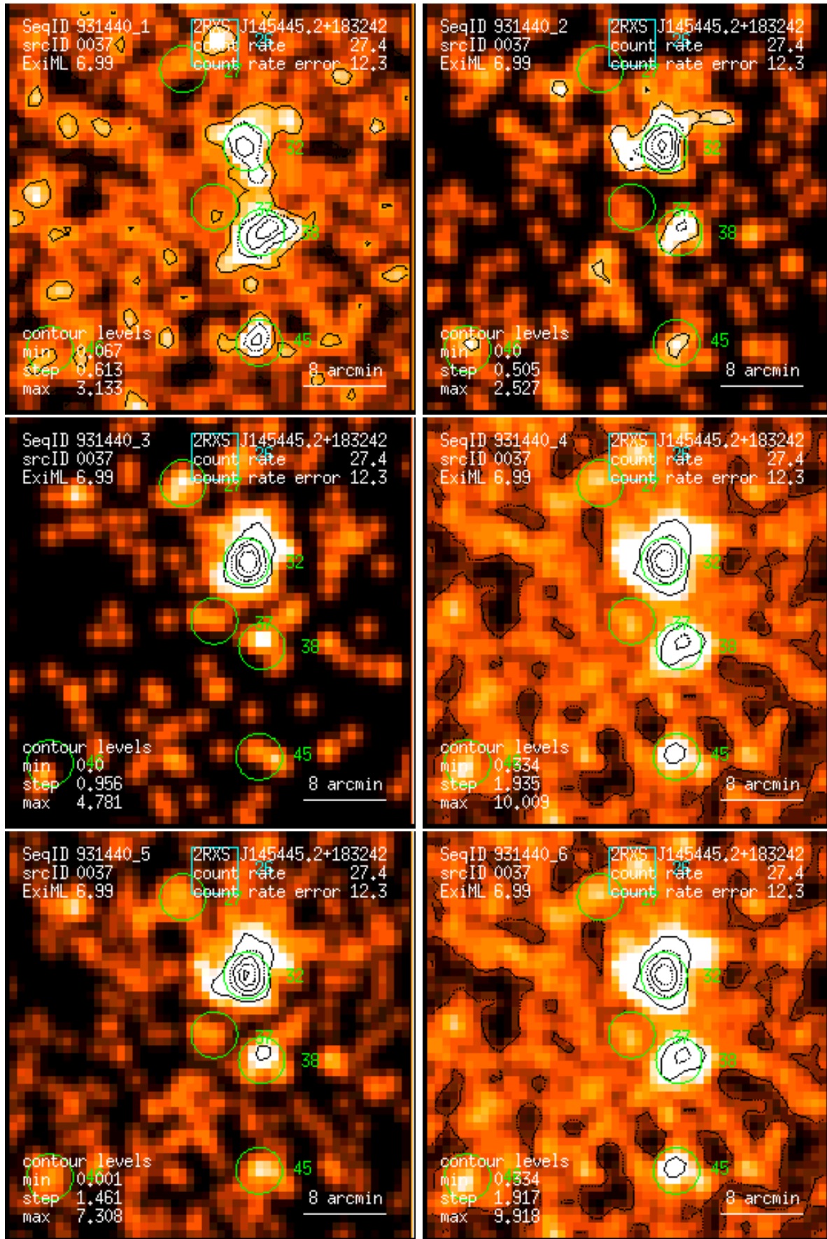
Figure 37: RASS 931440: detection 0037: band rate images, Gaussian filter: (1) PSPC channels 11 – 41, (2) 52 – 90, (3) 91 – 201, (4) 11 – 235, (5) 52 – 201, (6) 11 – 201. Broad band rates in counts/ks. Band rate contour levels in counts/ks/arcmin 2 .
