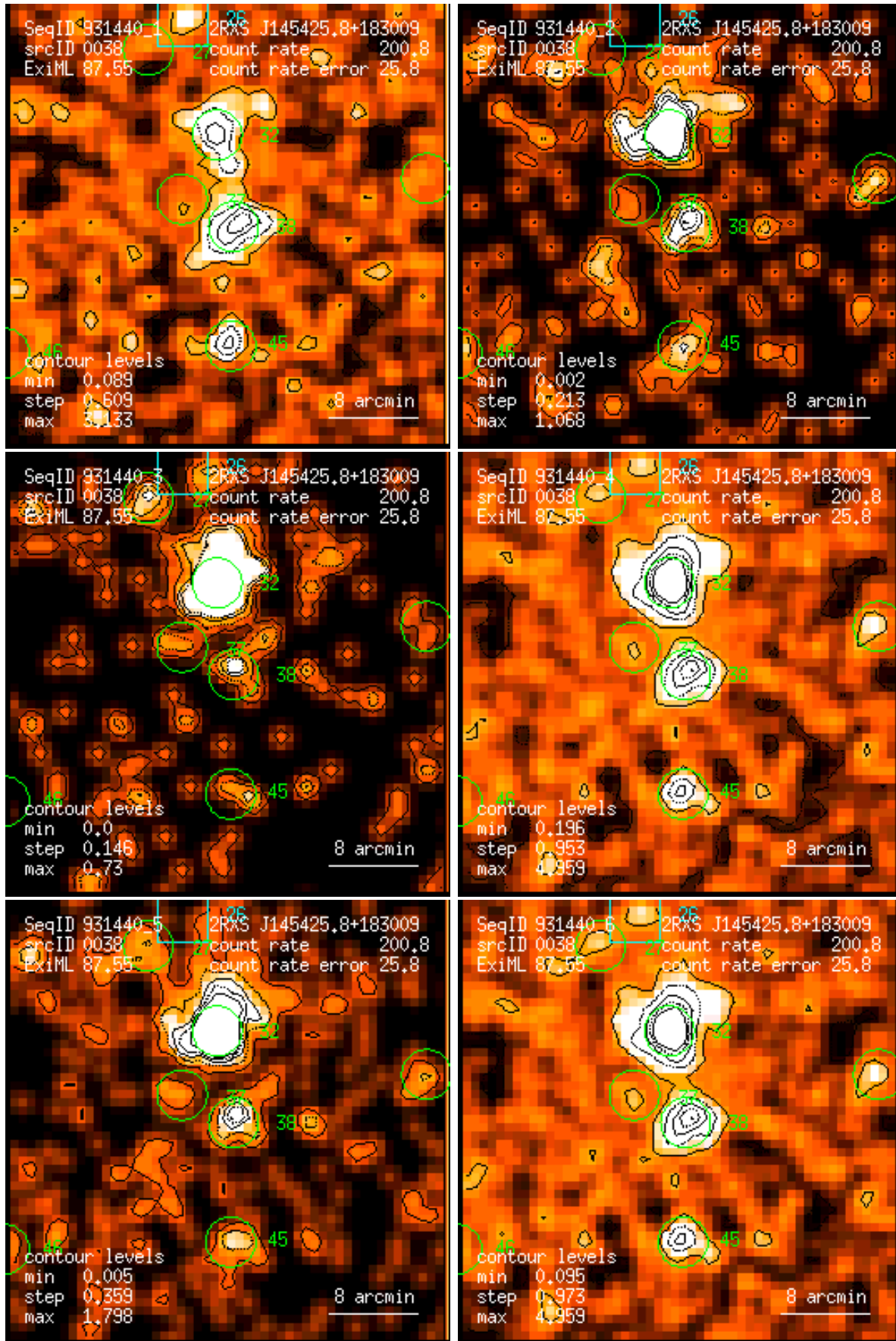
Figure 38: RASS 931440: detection 0038: band rate images, Gaussian filter: (1) PSPC channels 11 – 41, (2) 52 – 90, (3) 91 – 201, (4) 11 – 235, (5) 52 – 201, (6) 11 – 201. Broad band rates in counts/ks. Band rate contour levels in counts/ks/arcmin 2 .
