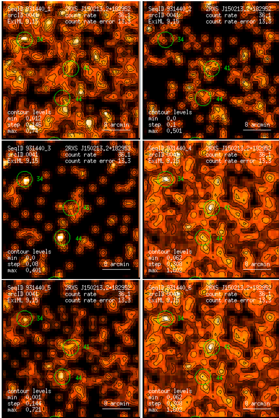
Figure 41: RASS 931440: detection 0041: band rate images, Gaussian filter: (1) PSPC channels 11 – 41, (2) 52 – 90, (3) 91 – 201, (4) 11 – 235, (5) 52 – 201, (6) 11 – 201. Broad band rates in counts/ks. Band rate contour levels in counts/ks/arcmin 2 .
