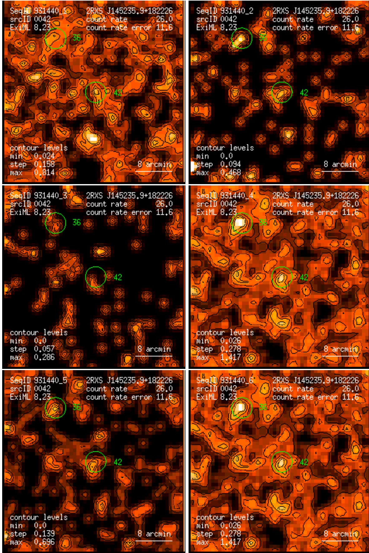
Figure 42: RASS 931440: detection 0042: band rate images, Gaussian filter: (1) PSPC channels 11 – 41, (2) 52 – 90, (3) 91 – 201, (4) 11 – 235, (5) 52 – 201, (6) 11 – 201. Broad band rates in counts/ks. Band rate contour levels in counts/ks/arcmin 2 .
