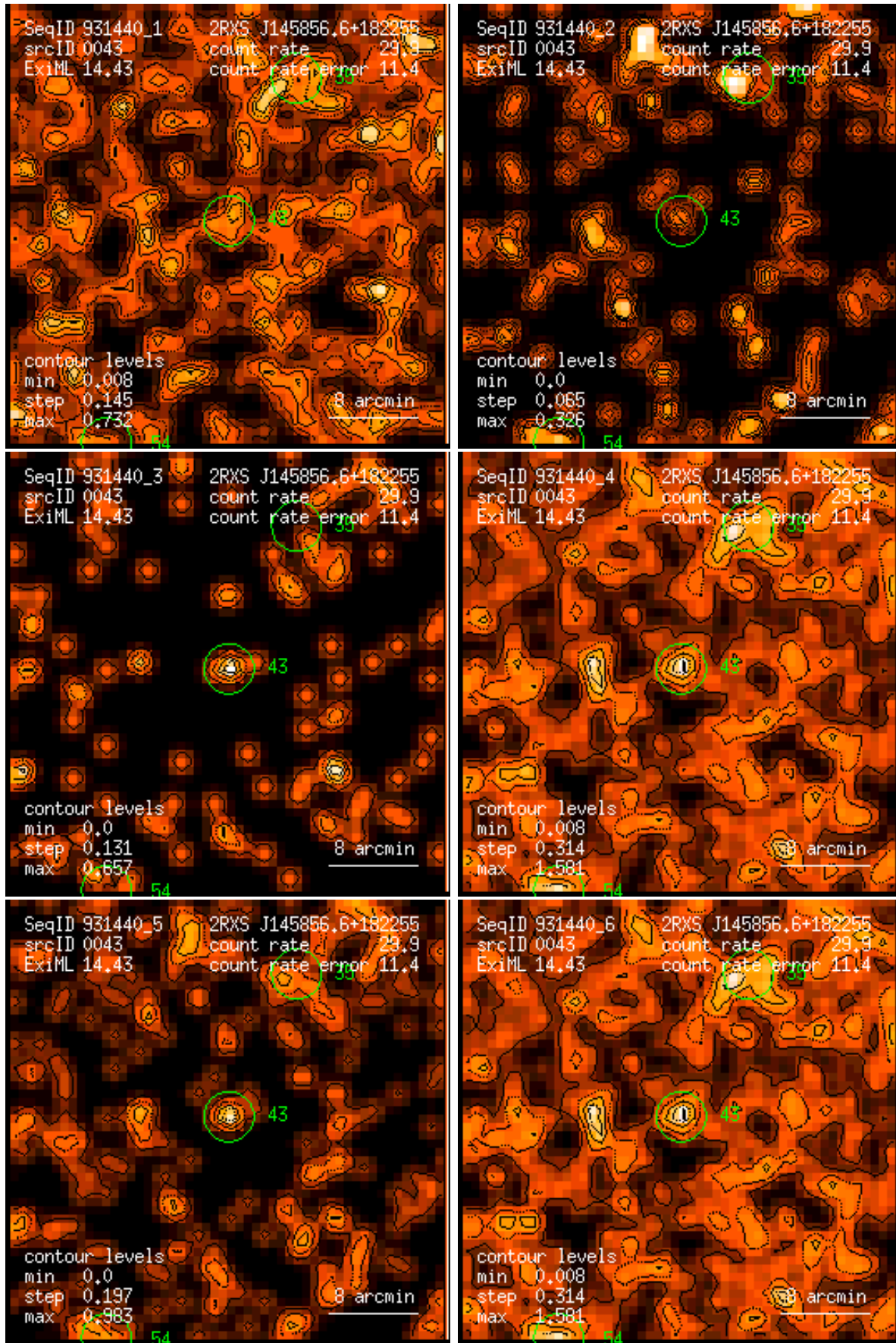
Figure 43: RASS 931440: detection 0043: band rate images, Gaussian filter: (1) PSPC channels 11 – 41, (2) 52 – 90, (3) 91 – 201, (4) 11 – 235, (5) 52 – 201, (6) 11 – 201. Broad band rates in counts/ks. Band rate contour levels in counts/ks/arcmin 2 .
